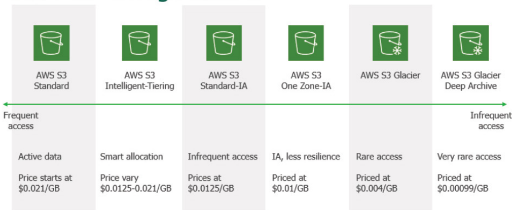
Figure 6. AWS S3 storage classes partial comparison
