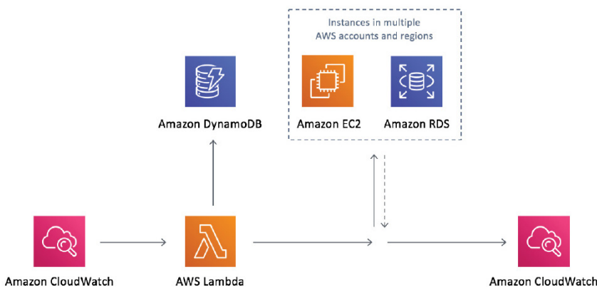
Figure 10. Amazon CloudWatch diagram
