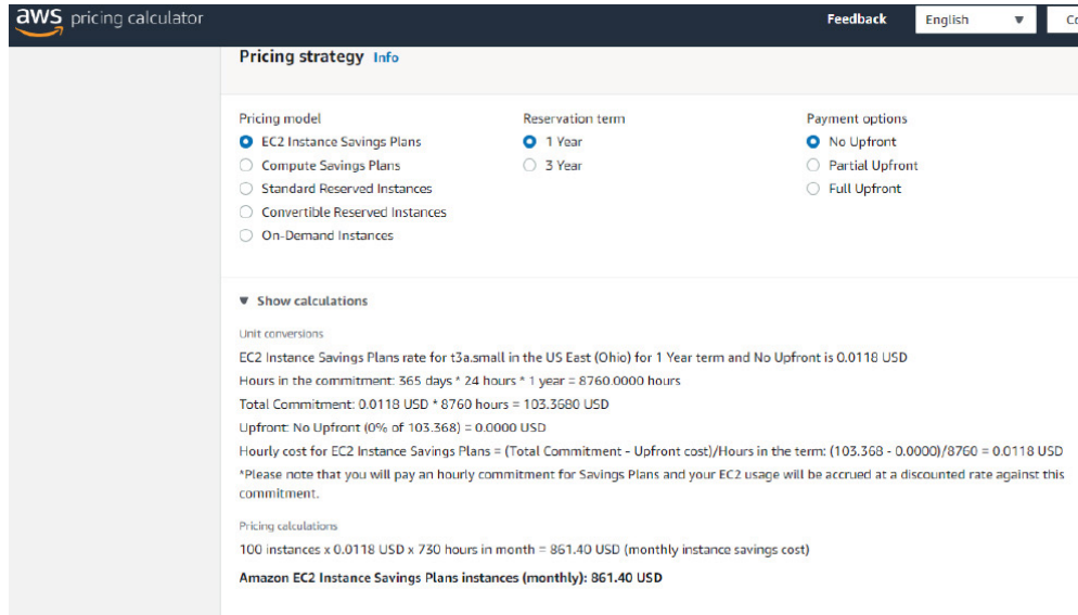
Figure 11. AWS pricing calculator cost prediction
