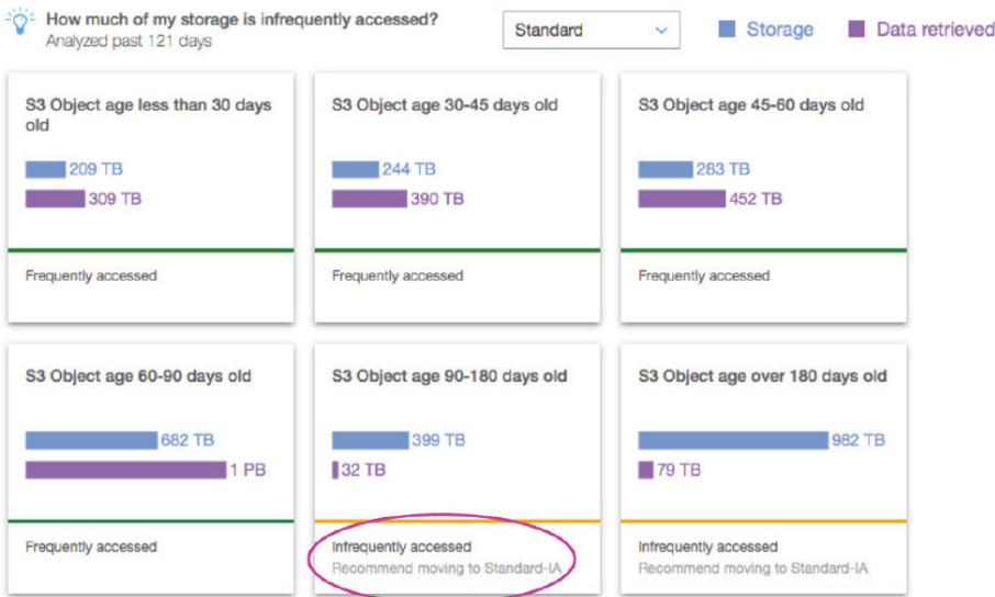
Figure 7. S3 bucket storage class analysis
