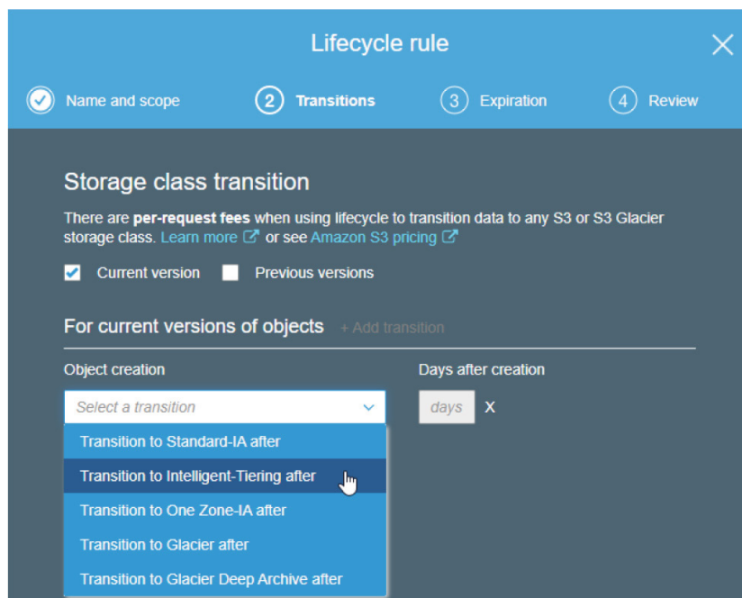
Figure 8. Lifecycle rule creation
