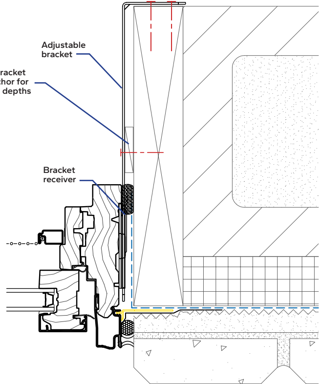
Wood Buck in Masonry Construction
