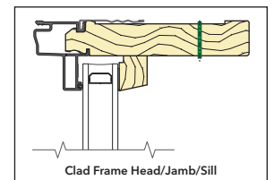
Clad Frame Head/Jamb/Sill
