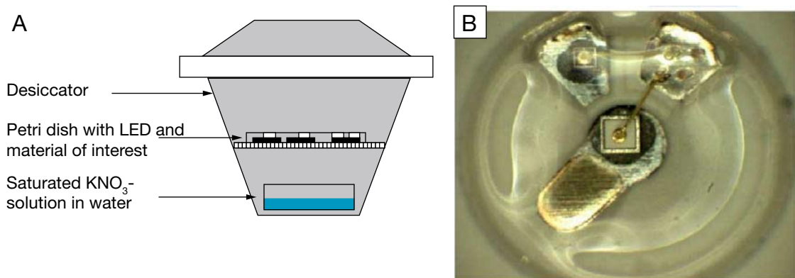
Figure 14: (A) Schematical description of device set-up for LED lead frame corrosion resistance test. (B) Example of a rubber-foam-incompatibility-affected LED lead frame
