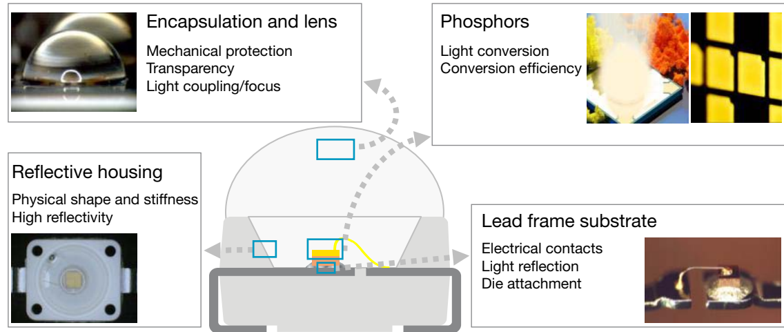
Figure 2: Overview of four LED package materials
