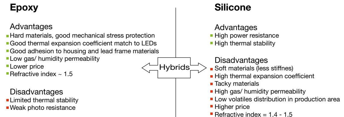
Figure 8: Brief summary of certain epoxy, hybrid and silicone properties
