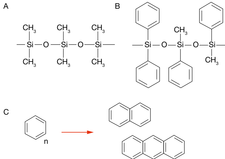
Figure 10: Two examples of silicone: (A) dimethylsiloxanes. (B) phenylsiloxanes. (C) Cleaved (phenyl) aromatic side groups from a silicone can react with each other and form chromophores, which may cause silicone discoloration
