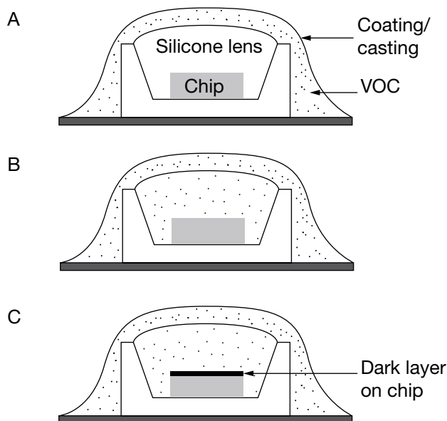
Figure 11: Schematic scenario of VOC-involved encapsulation discoloration
