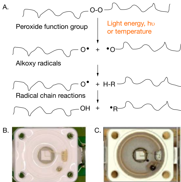
Figure 3: (A) Concept of thermal oxidation and free radical formation. (B) and (C) A thermoplastic-based housing material before (B) and after (C) discoloration. Material degradation shown in (C) results in a visibly yellow-brown appearance. The affected region is more pronounced in the area close to the center chip, as the luminance flux is much higher. This discoloration decreases overall light output due to poor function of the yellow-to-brown reflector
