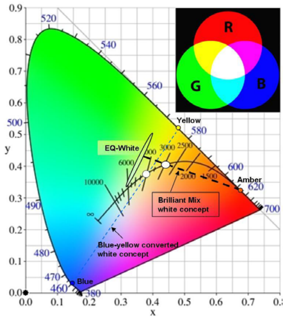
Figure 5: Principles of color mixing
