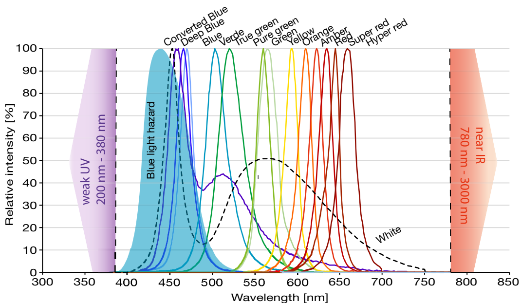
Figure 4: Typical spectra of high-power LEDs from ams-OSRAM AG
