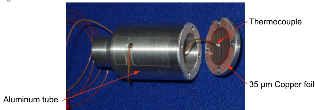
Figure 9: Measurement device
