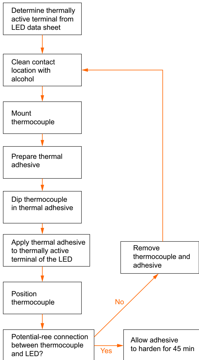
Figure 4: Process overview: Mounting the thermocouple to an LED
