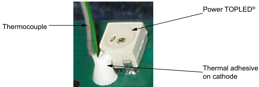
Figure 3: Thermocouple attached to a Power TOPLED®
