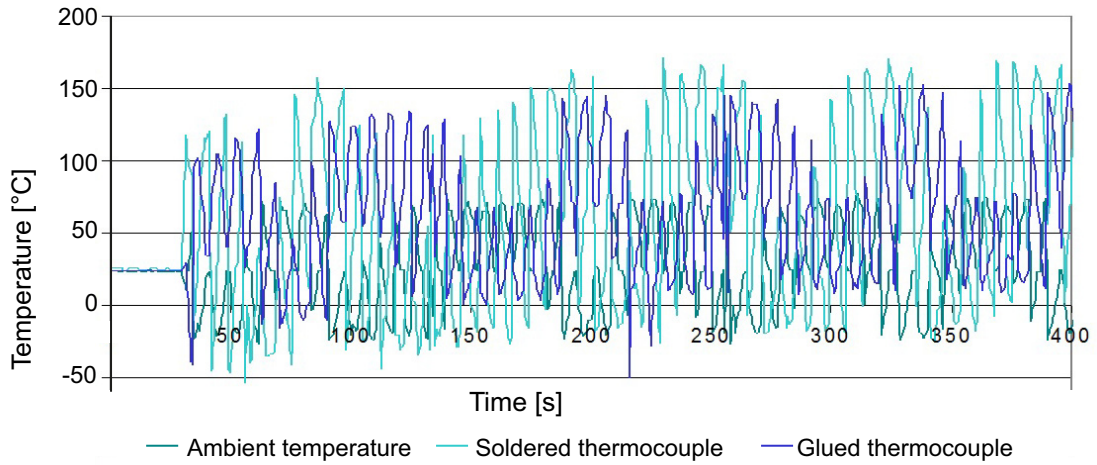
Figure 5: Switching power supply without electrical isolation from power line
