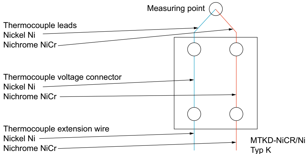
Figure 8: Principle arrangement of thermal clamps
