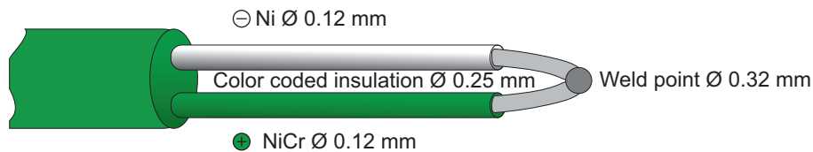
Figure 2: Thermocouple of type K
