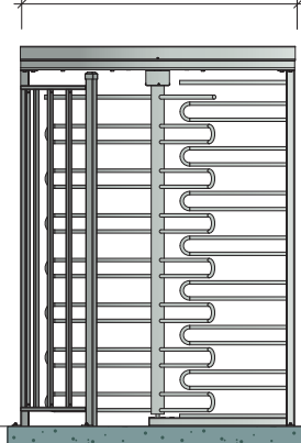
Front View 1620
