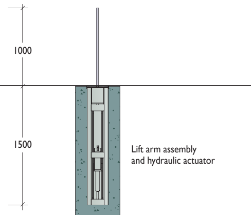
Side View 282
