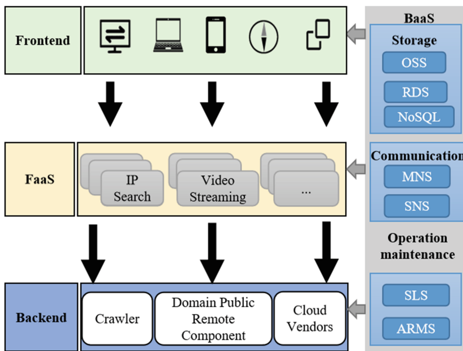
Fig. 5 The Structure of the Serverless Design
