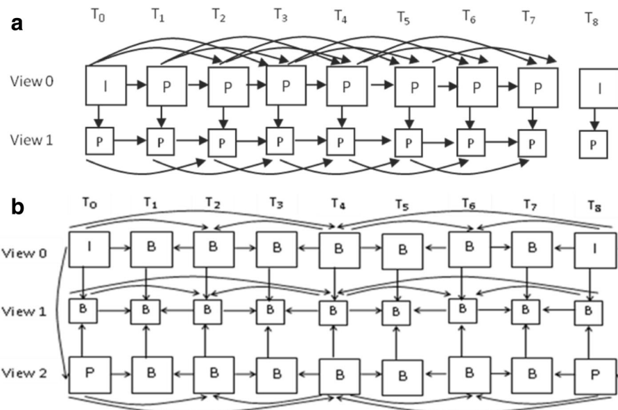
Fig. 1 Prediction architectures. a 3D-DMB. b Hierarchical B-picture
