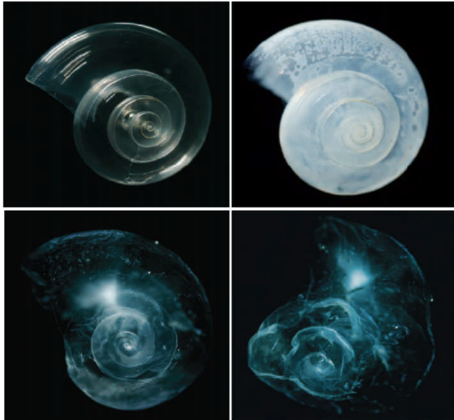
Figure 12: Dissolution of pteropod shell in higher acidity water. Dissolution occurred over 45 days in waters with pH and carbonate levels expected at the end of the century 28 .
