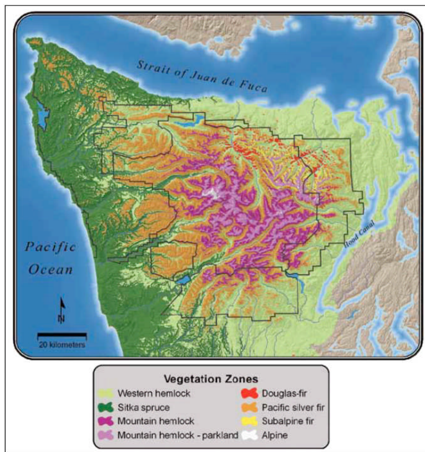
Figure 14: Vegetation zones on the Olympic Peninsula 31 .
