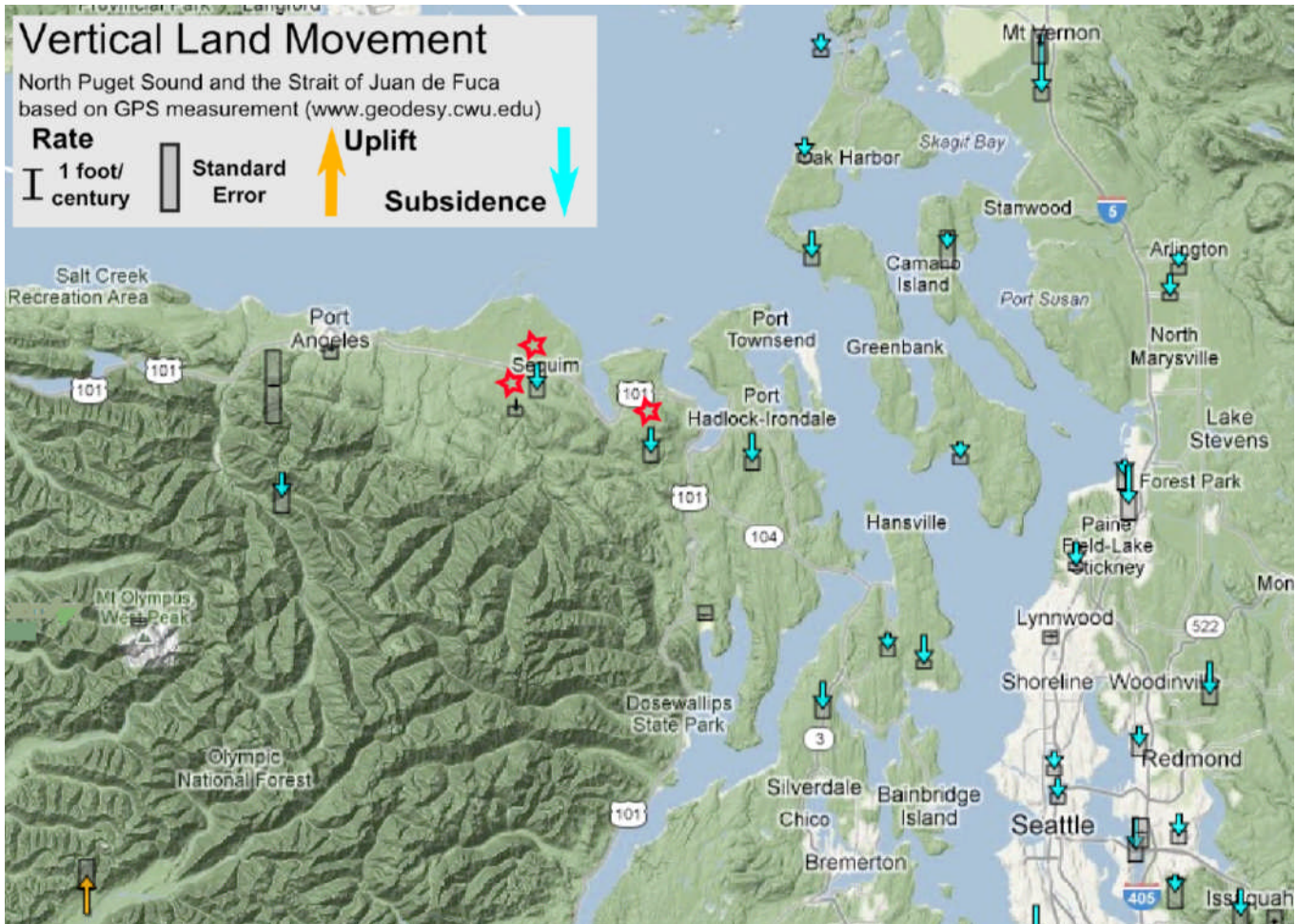
Figure 9: Rates of vertical land movement for sites adjacent to Sequim Bay. Continuous GPS sites in the Pacific Northwest monitor rates of vertical land movement. Orange arrows represent land that is uplifting (rising). Blue arrows represent land that is subsiding (sinking). Red star mark the three sites used to estimate average subsidence in this assessment (Table A-1).
