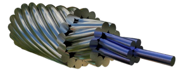
Figure A-109. ACSS conductor.
