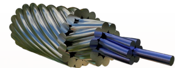
Figure A-44. ACSS conductor.
