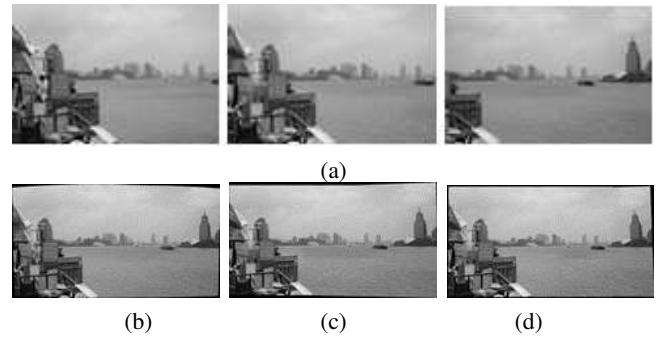
Fig. 7: Image Stitching. First row: (a) Input images from the Shanghai dataset. Second row: (b) Brown and Lowe [33], (c) Gao et al. [91], and (d) SIASM [163] (Images from Li and Monga [163]).
