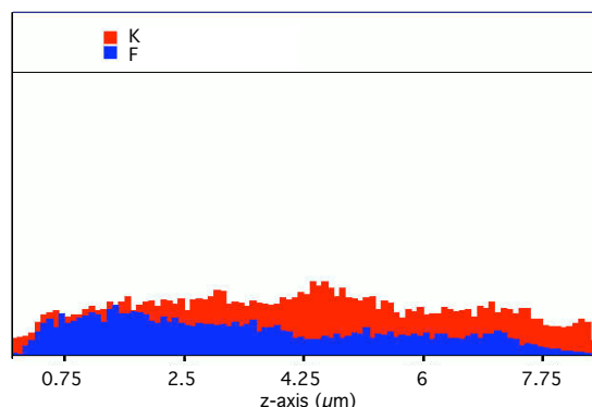
Fig. 8. Cross-section EDS profiles (red: potassium, blue: fluorine atoms) of PVDF-g-PAA films initially electron irradiated at 100kGy, radiografted at 60°C for 1 h (AA concentration 5%v/v, grafting yield 9%w/w) with 0.25%w/w of Mohr's salt and treated in solution of tBuOK (50%w/w).
