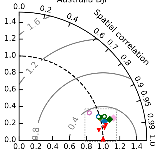
Australia DJF
