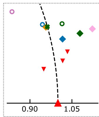
Australia DJF
