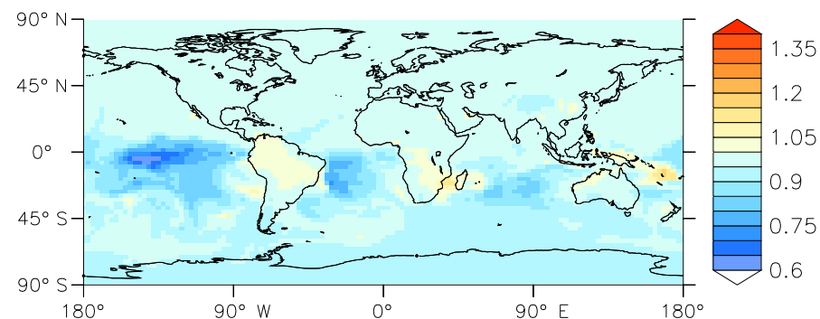
(c) POLY/FULL: ozone ratio
