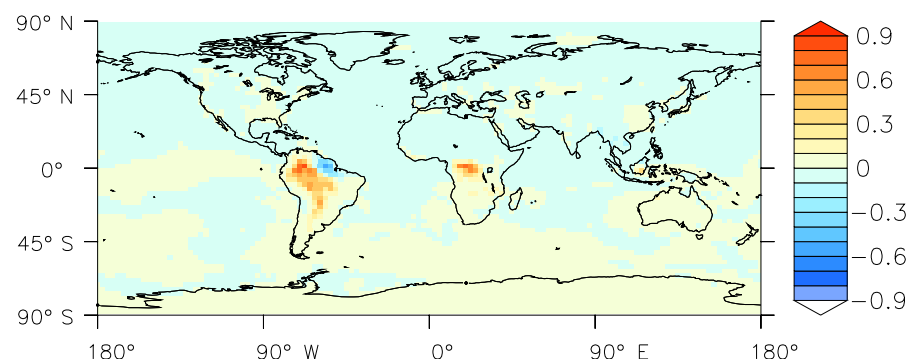
(f) SKEL-FULL: isoprene difference (nmol mol -1 )
