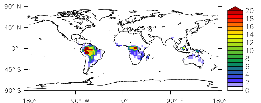
(b) FULL: isoprene (nmol mol -1 )
