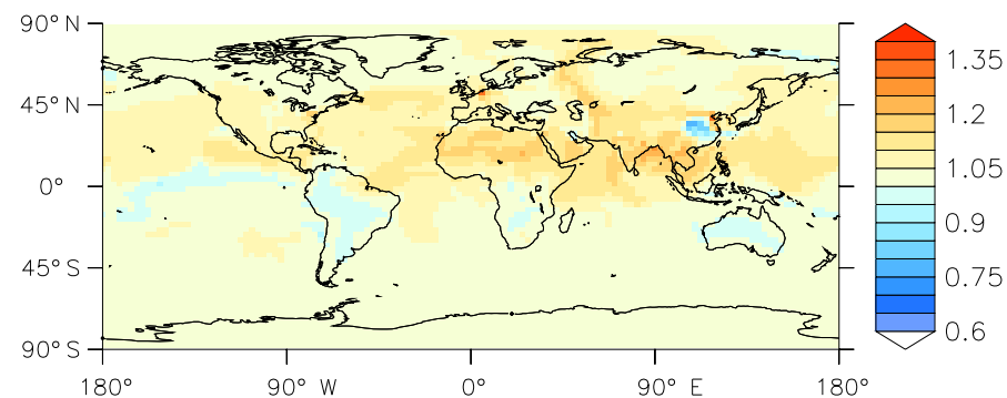
(e) SKEL/FULL: ozone ratio
