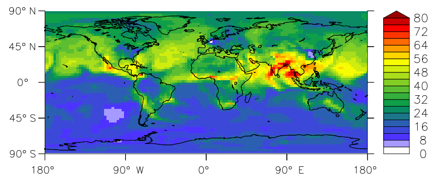
(a) FULL: ozone (nmol mol -1 )
