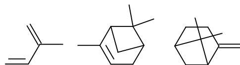
Isoprene Alpha-pinene Beta-pinene
