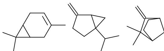
3-carene Sabinene Camphene
