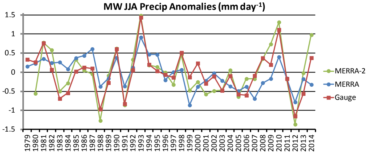
Figure 6-16 Time series of Midwestern US summer seasonal precipitation anomalies, following Bosilovich (2013). The anomalies are from the 1980-2011 JJA mean. The gauge data are from CPC gridded daily data for the US (Chen et al. 2008; Xie et al. 2007). MERRA-2 precipitation is from the model-generated fields.
