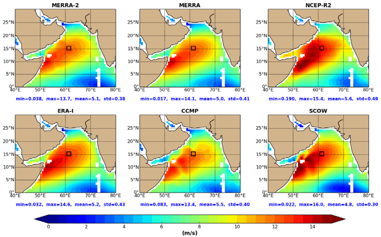
Figure 8-14 Monthly mean of 10-meter wind speed in the Arabian Sea for July 1995. Black square shows the location of the time-series in Figure 8-13.
