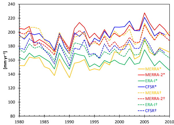
Figure 9-7 As in Figure 9-5 but for the region 70S to 90S, in \text{mm yr}^{-1} .
