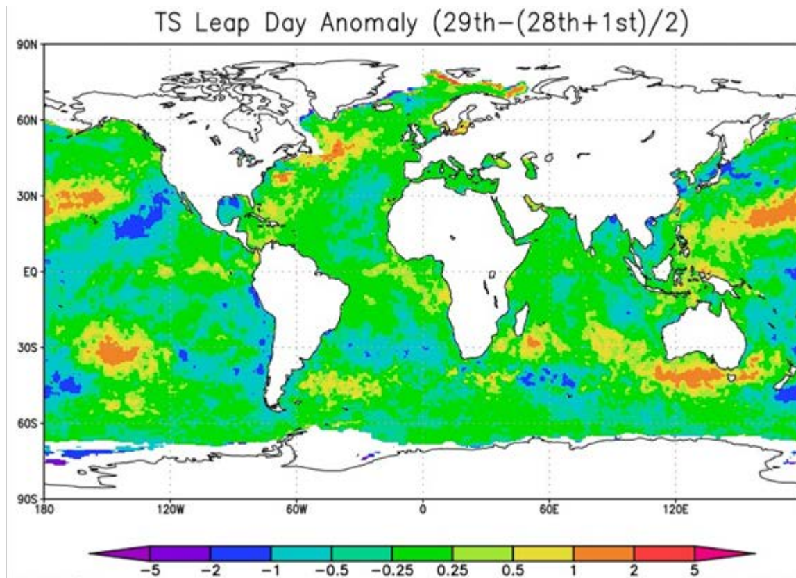
Figure 8-4 SST anomaly (K) on 29 February 1980 compared to the average of the previous and next days.
