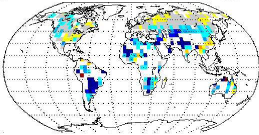
a) MERRA – HadISDH q^{2m} [g/kg]
