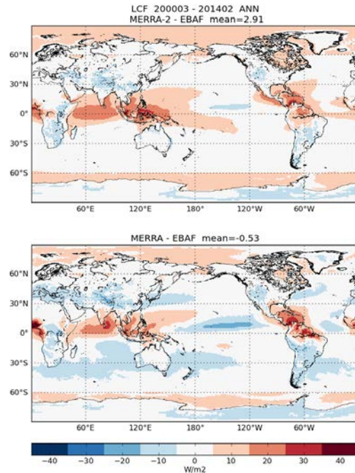
Figure 5-6 The corresponding (to Figure 5-5) differences: MERRA-2 minus EBAF (top) and MERRA minus EBAF (bottom).
