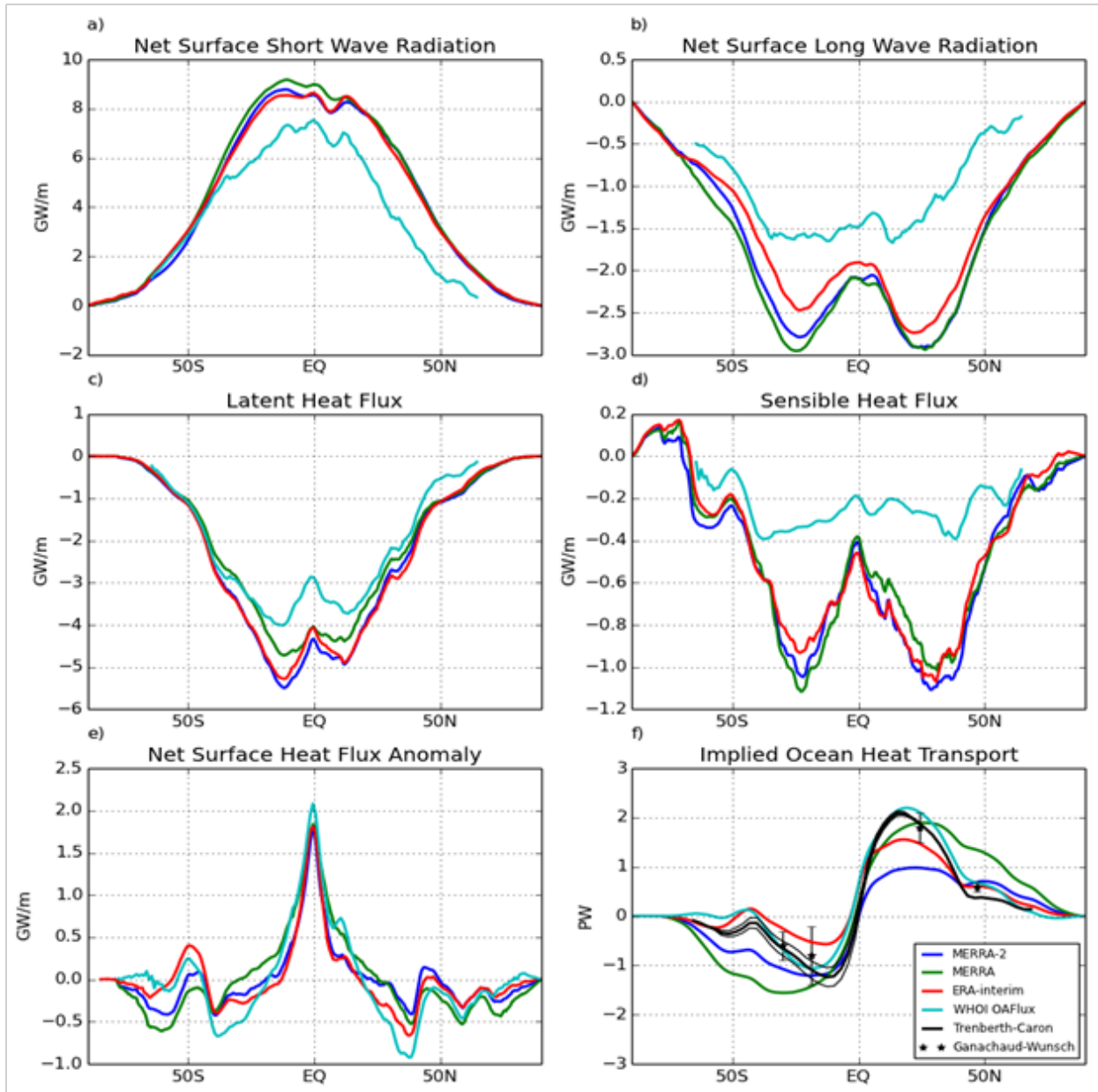
Figure 4-7 Zonally integrated time mean ocean surface fluxes (a-e) in giga-watts per meter for MERRA, MERRA-2, ECMWF ERA-Interim reanalyses and WHOI OAFflux objective analysis. (a) Net surface shortwave radiation; (b) net surface long wave radiation; (c) latent heat flux; (d) sensible heat flux; (e) net surface heat flux anomaly (global mean removed). (f) Implied northward ocean heat transport in peta-watts for MERRA, MERRA-2, ECMWF ERA-Interim, and WHOI OAFflux along with estimations from Trenberth and Caron (2001) and Ganachaud and Wunsch (2000).
