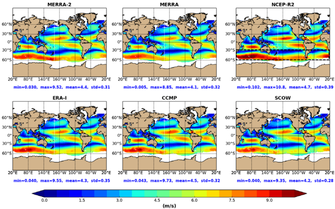
Figure 8-9 Mean 10-meter wind speed ( m s^{-1} ), 1999-2009.
