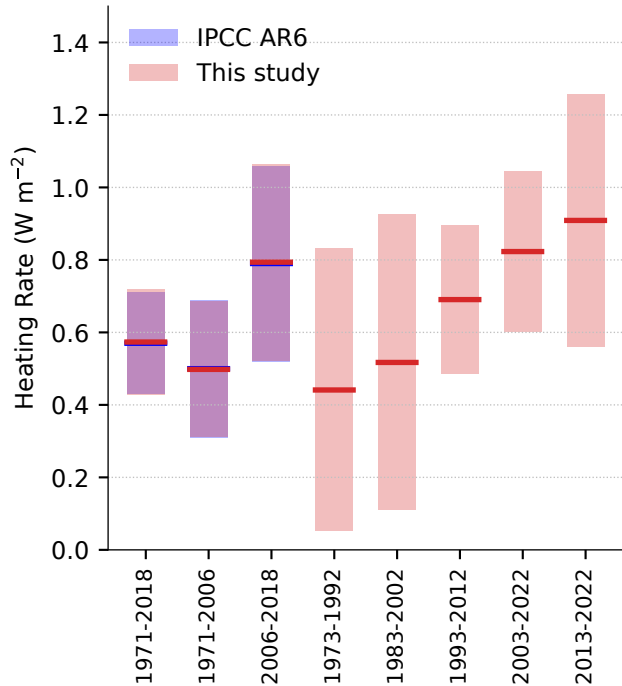
(b) Earth Energy Imbalance
