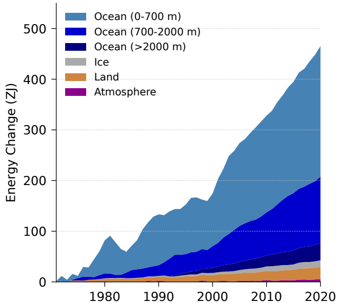
(a) Earth Heat Inventory
