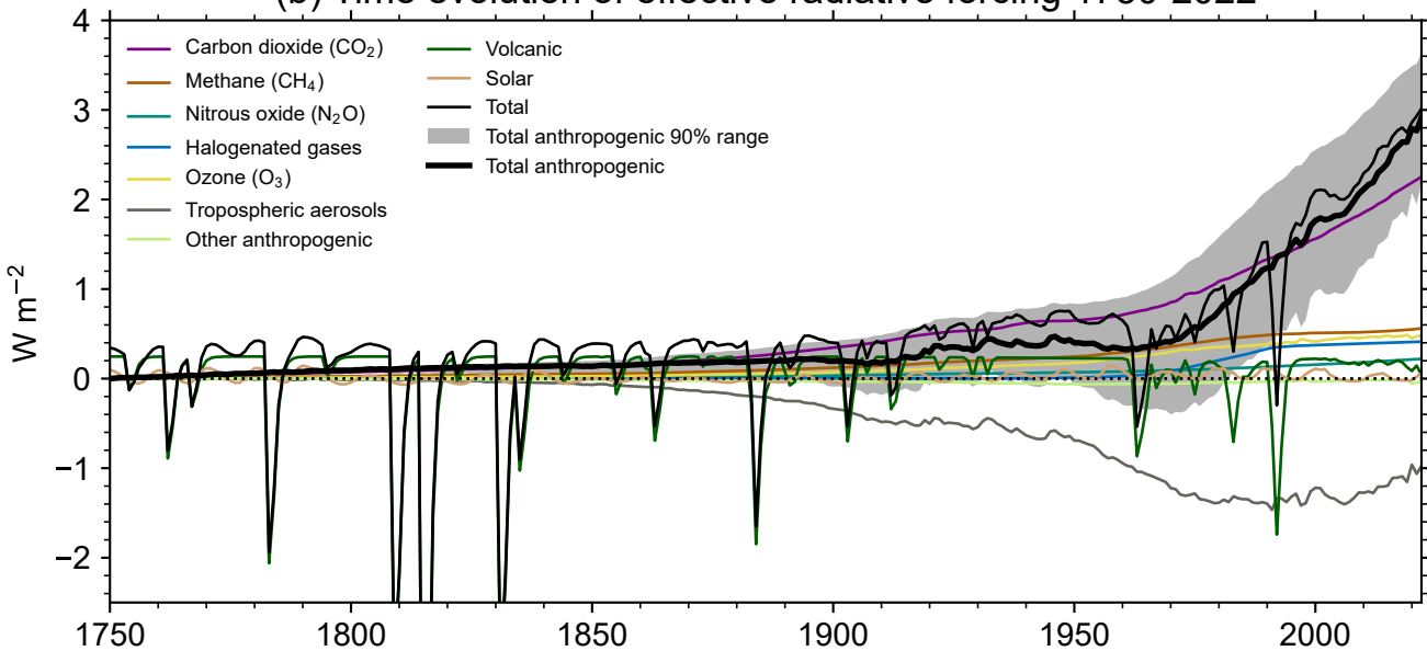
(b) Time evolution of effective radiative forcing 1750-2022
