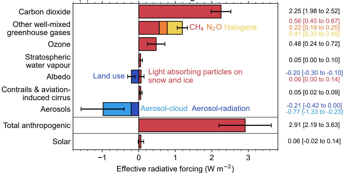
(a) Effective radiative forcing from 1750 to 2022
