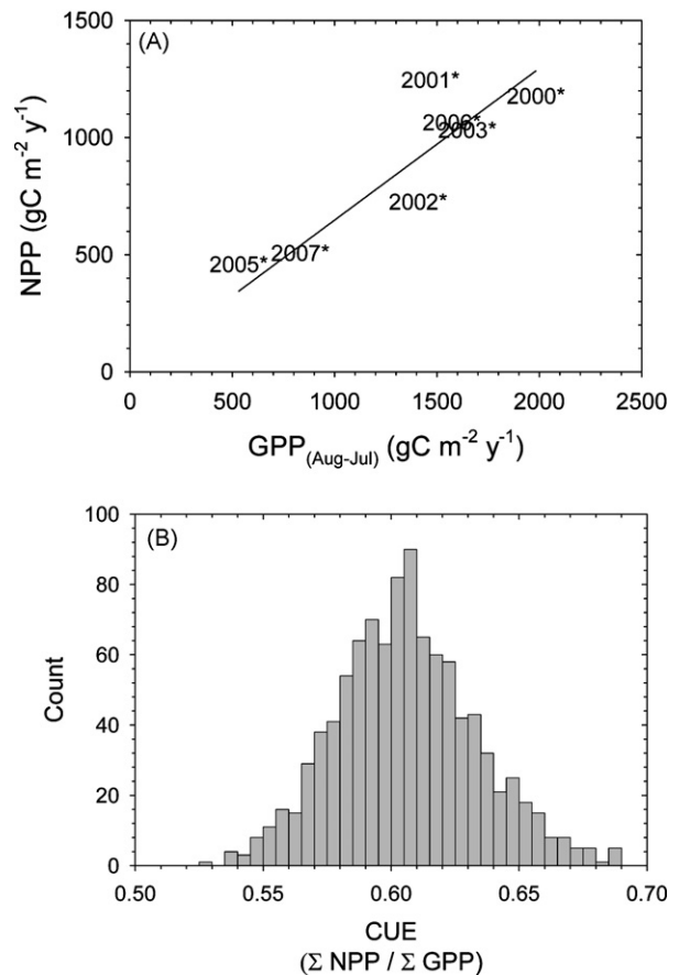
Fig. 2 – Relationship between NPP and GPP from the previous year's August to the current year's July ( NPP = 0.65GPP ; r^2 = 0.76 ; p = 0.01 ) at the SJFM (A). Histogram of the 1000 bootstrapped estimates of the SJFM's carbon use efficiency ( NPP/GPP ) (B).
