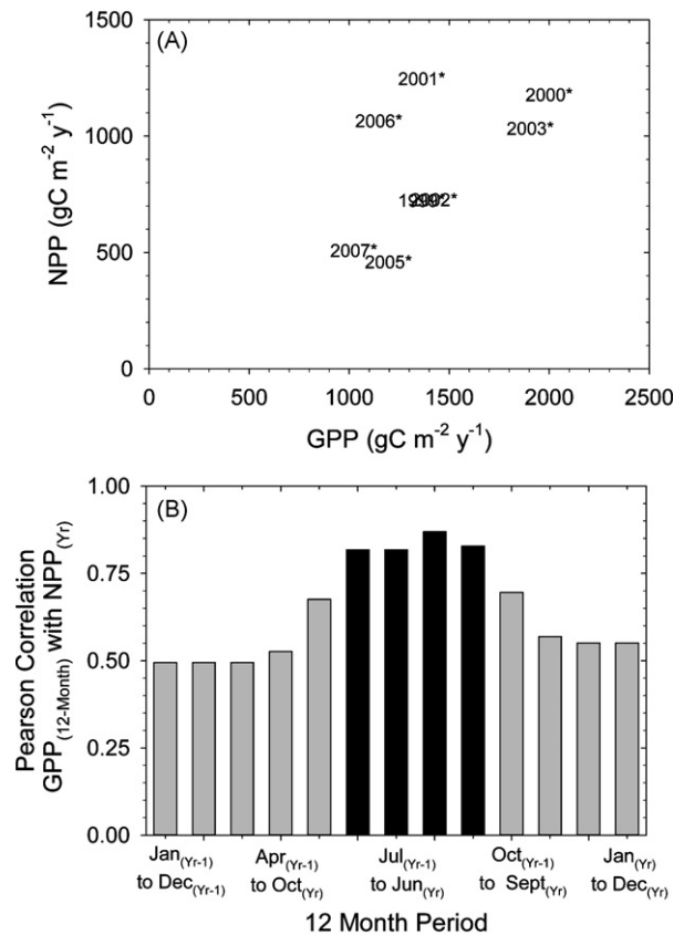
Fig. 1 – Relationship between annual GPP and NPP for the SJFM (A) ( r^2: 0.33; p: 0.14 ). Pearson correlation coefficients for NPP and GPP calculated using a 12-month period lagged with a time step of a month (B). Black bars denote statistically significant relationships at the 95% confidence level.
