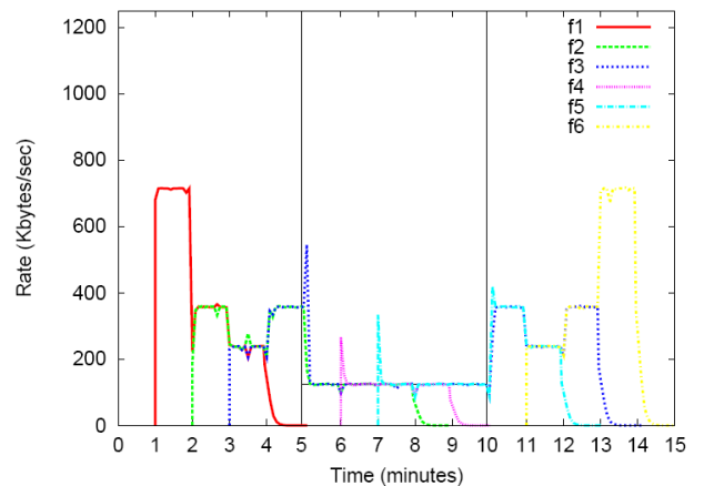
Figure 3. Those iperf flows that are active during the 300-second time window (vertical lines in the graph) are rate-limited to 1Mbps
