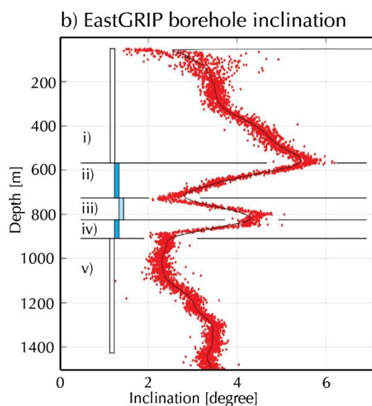
45 Fig. 1: a) The inclination correction tool, a spring attached to the outer barrel, designed on-site to decrease borehole inclination at the EastGRIP in 2018. b) Borehole inclination of the upper 1500 m of the EastGRIP hole (pers. comm. Dorthe Dahl-Jensen). Section i) To increase the descent speed of the drill, a deadweight was added to the lightweight short version of the deep drill. This caused the drill's center of gravity to be above the supporting knobs, leading to a rise in the inclination when drilling. ii) We mounted the inclination spring and repositioned the support knobs, gradually decreasing the inclination. iii) We mounted the spring the wrong way around and the inclination increased again. iv) We mounted the spring in the right way again. v) We removed the spring 50 as the inclination was now acceptable.
