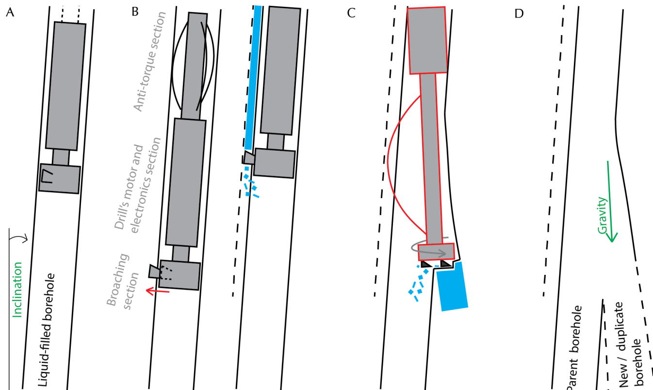
70 Figure 2: Concept of the directional drilling setup. A) the broaching tool is lowered into the liquid-filled and slightly inclined borehole. B) The cutter is engaged into the borehole wall (red arrow), and then the tool is pulled up, cutting a groove into the side of the wall. C) The broaching tool is replaced by the spring sleeve and the spring follows the groove (dashed line). The milling head cuts into the side of the borehole wall. D) When lowering the ice core drill, gravity will guide it into the new borehole. In our test we did not perform step D, but stopped at step C.
