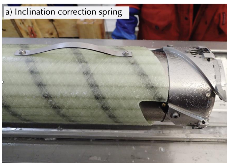
45 Fig. 1: a) The inclination correction tool, a spring attached to the outer barrel, designed on-site to decrease borehole inclination at the EastGRIP in 2018. b) Borehole inclination of the upper 1500 m of the EastGRIP hole (pers. comm. Dorthe Dahl-Jensen). Section i) To increase the descent speed of the drill, a deadweight was added to the lightweight short version of the deep drill. This caused the drill's center of gravity to be above the supporting knobs, leading to a rise in the inclination when drilling. ii) We mounted the inclination spring and repositioned the support knobs, gradually decreasing the inclination. iii) We mounted the spring the wrong way around and the inclination increased again. iv) We mounted the spring in the right way again. v) We removed the spring 50 as the inclination was now acceptable.
