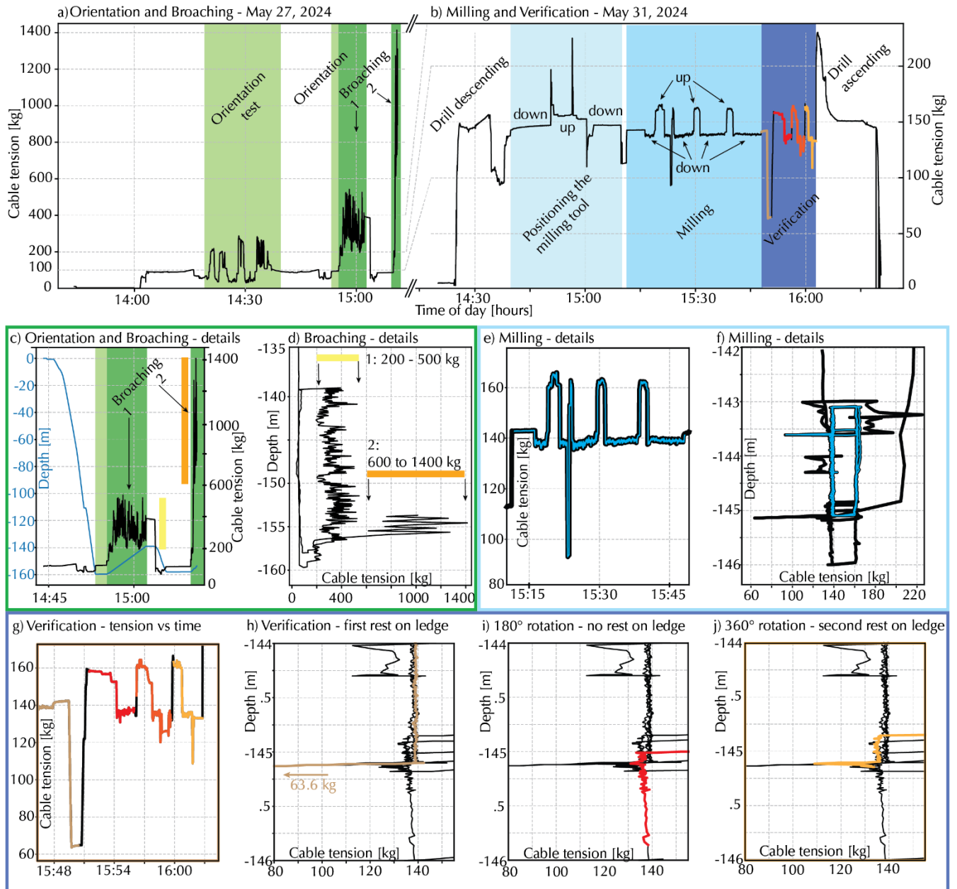
90 Figure 3: a, b) Overview of the orientation, broaching, milling, and verification run. c, d) show the broaching procedure in detail, including the stick-slip of the broaching tool and the resulting cable tension, e, f) the procedure of the milling process. g-j) show the plots of the verification of having cut a ledge, by reducing the cable tension by resting the drill on the newly cut ledge.
