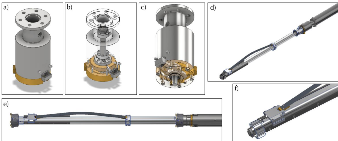
115 Figure 4: a, b, c) The broaching tool in detail. d) The optional spring below the broaching tool. e,f) The milling head can be mounted either at the bottom or top of the spring sleeve, facing down (cut while descending) or facing up (cut while ascending). Only one milling head would be mounted at a time. The linear rail at the bottom of the spring can be limited in travel to produce lateral force, either by a bolt as shown above, or a spring for longer travel demands.
