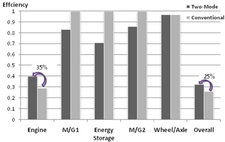
Figure 5-40 Efficiency of Two Mode HEV and Conventional ICE Vehicle on HWFET Cycle
