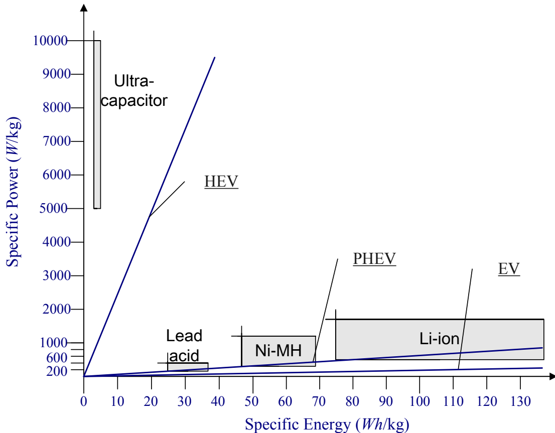
Figure 2-1 Power/Energy Ratio of Vehicle Demand and ESS Capability
