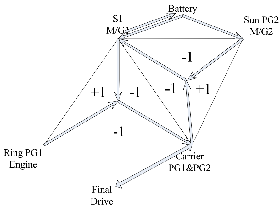
Figure 5-17 Power Flow of Second Mode at a Vehicle Speed Greater than V_{s3}
