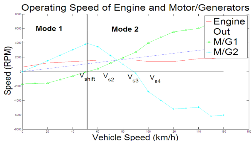
Figure 5-26 Speed Profile of All Shafts (Engine Speed predefined)
