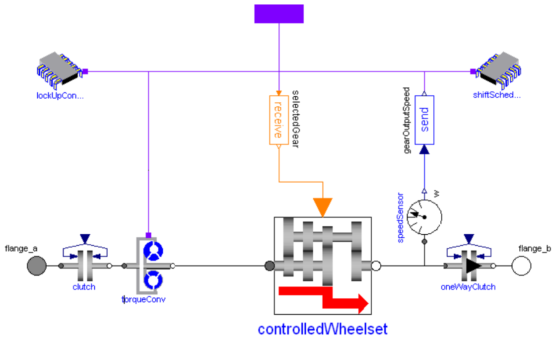
Figure 6-6 Transmission Model in Dymola
