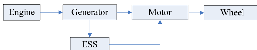
Figure 1-3 a Series Hybrid Electric Vehicle Configuration
