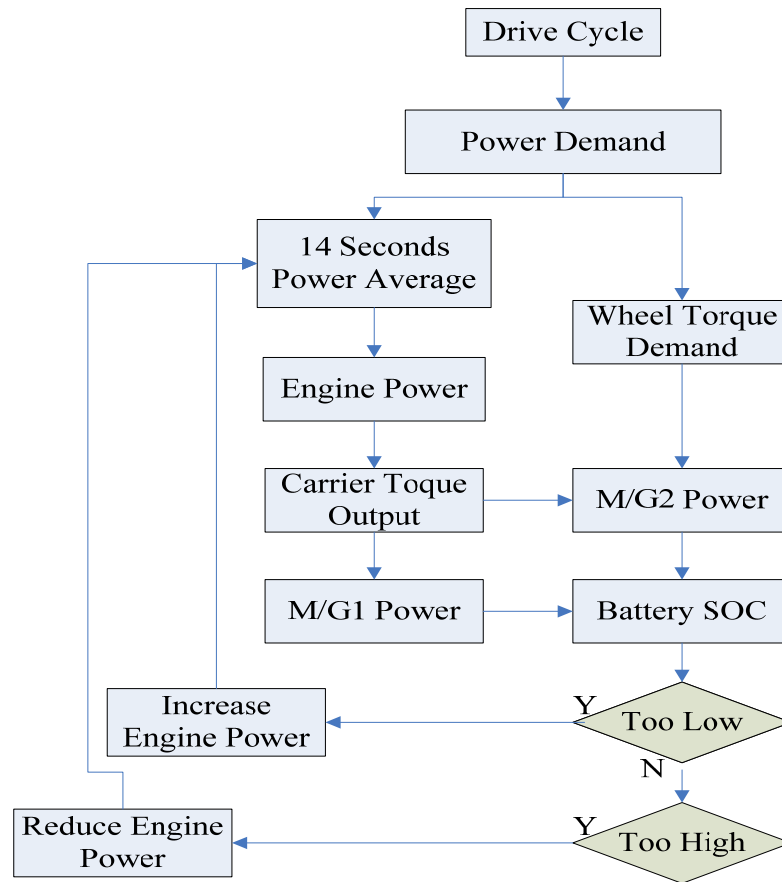
Figure 5-27 Power Management Chart Mode 1
