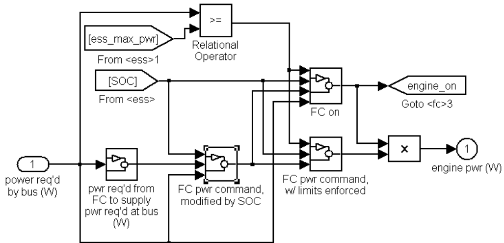
Figure 4-6 a Fuel cell system Model in ADVISOR
