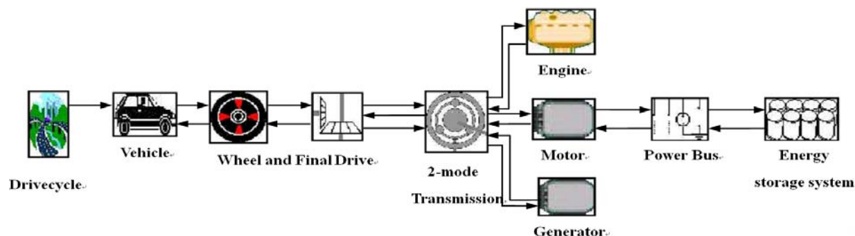
Figure 3-2 ADVISOR/Simulink Block Diagram of a Two-mode Truck
