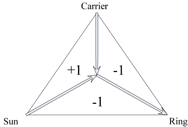
Figure 5-2 Power Flow Chart of Planetary Gear
