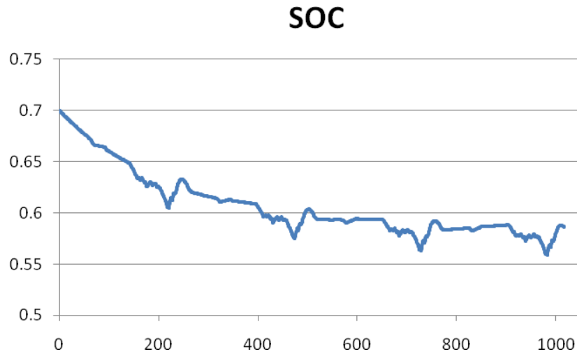
Figure 5-36 Battery SOC History on NYCTRUCK
