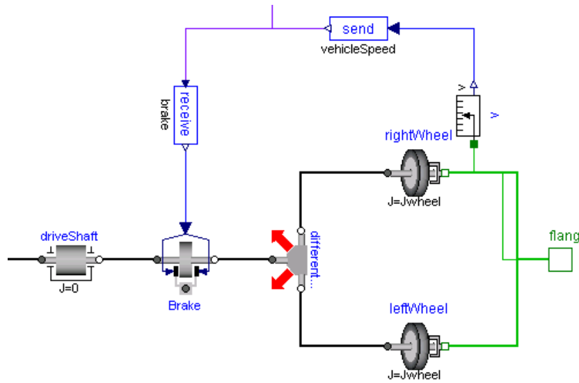
Figure 6-7 Chassis Model in Dymola
