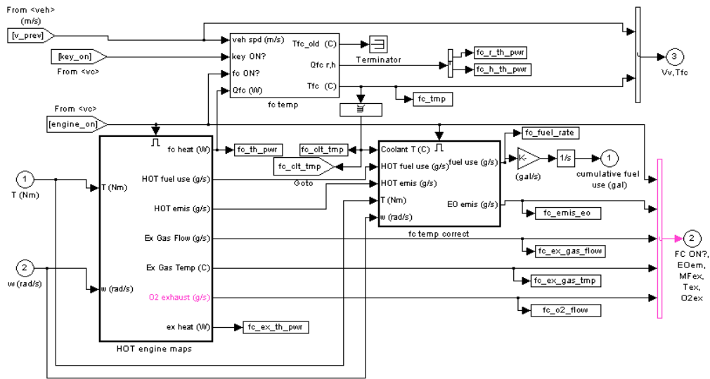
Figure 5-21 Simulink Block Diagram of Engine Thermal and Fuel Model
