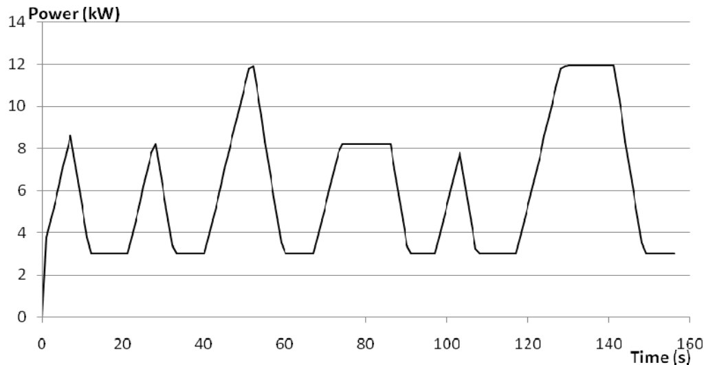
Figure 4-17 Fuel cells Power Demand-Low Power Cycle
