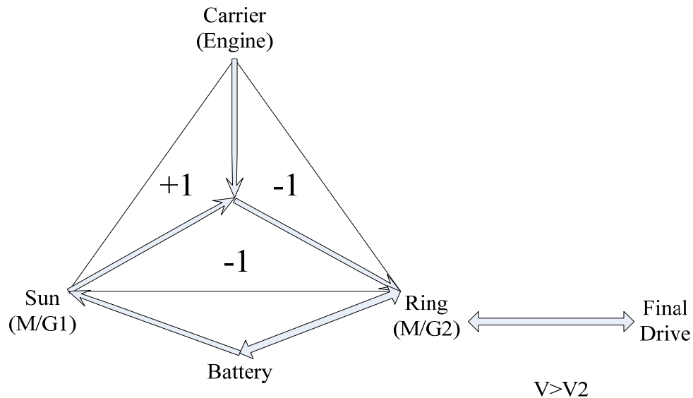
Figure 5-8 THS Power Flow Chart V > V_2
