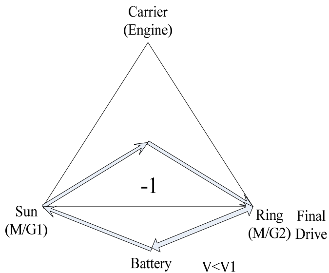
Figure 5-5 THS Power Flow Chart Engine Off
