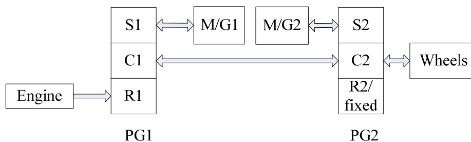
Figure 5-9 First Mode Drivetrain Configuration
