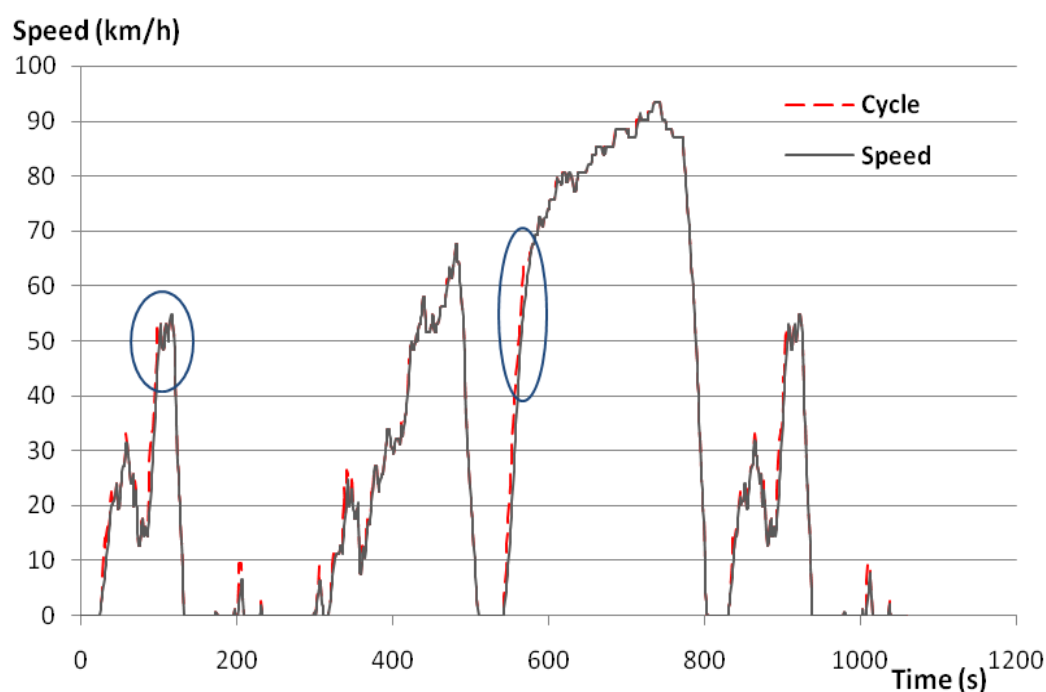
Figure 5-29 Vehicle Speed on the UDDSHEV Cycle
