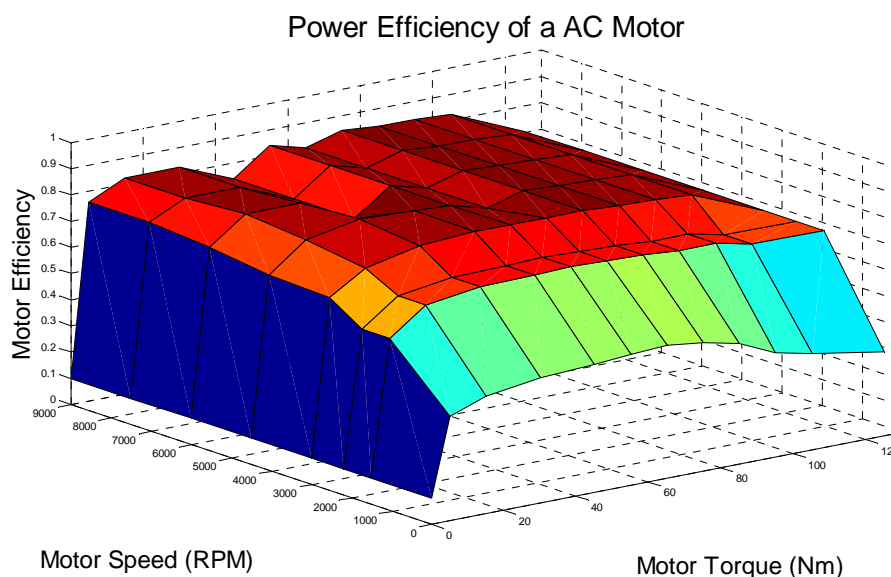
Figure 4-10 AC30 Motor Power Efficiency
