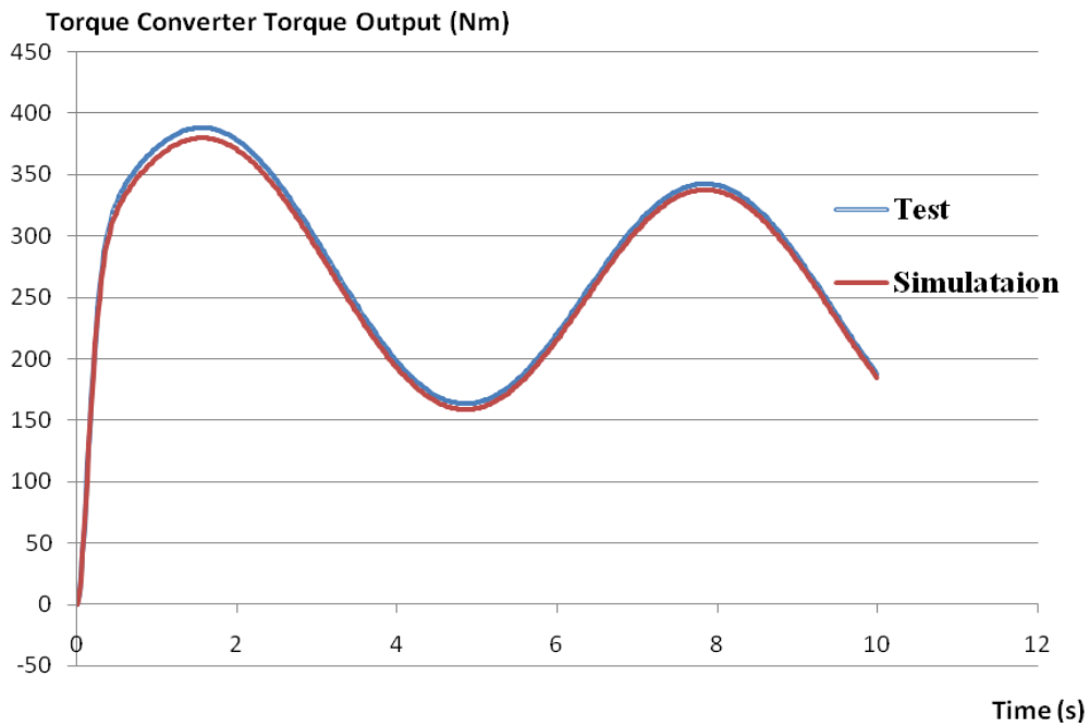
Figure 6-11 Torque Converter Validation - Output Torque
