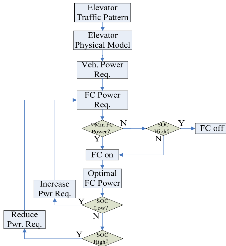
Figure 4-14 Fuel cell system Power Management Flow Chart
