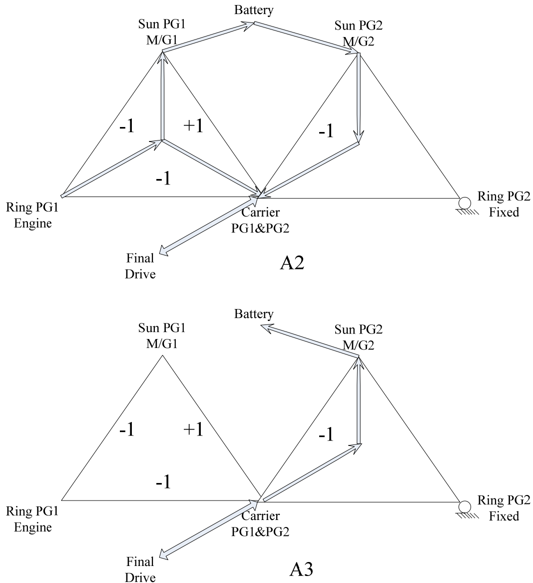
Figure 5-12 Power Flow Chart of Forward Movement in the First Mode
