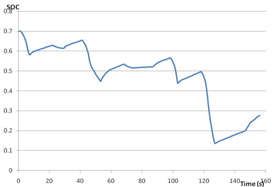
Figure 4-24 Ultracapacitor SOC-High Power Cycle
