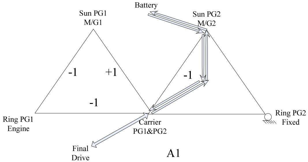
Figure 5-11 First-mode Power Flow Chart-Engine Off
