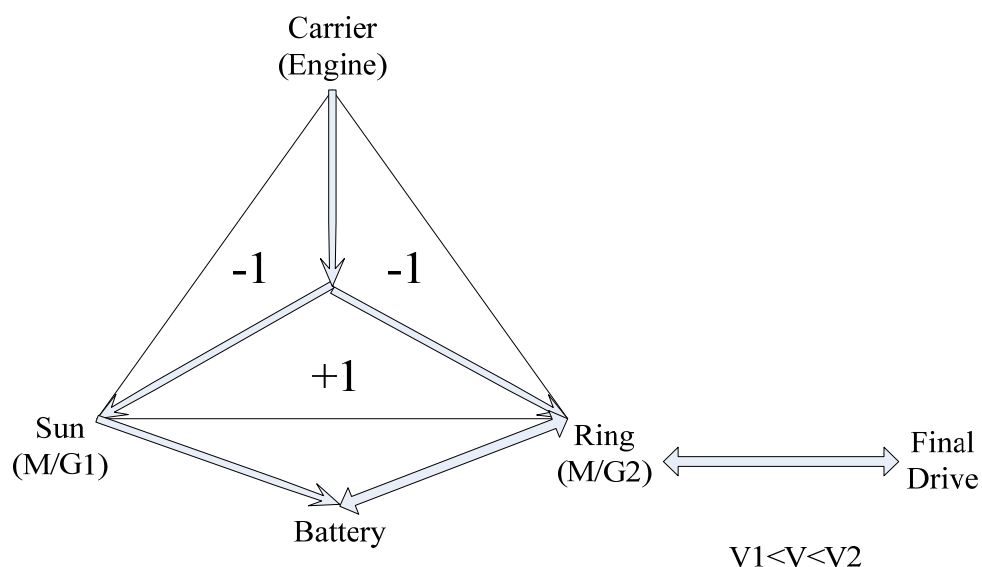
Figure 5-7 THS Power Flow Chart V_1 < V < V_2
