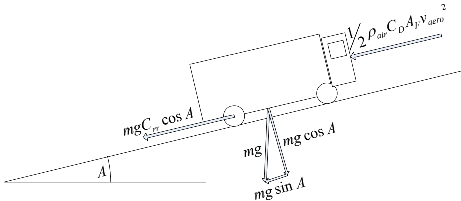
Figure 5-19 Free Body Diagram of a Truck
