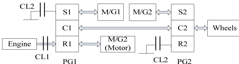
Figure 5-22 A Schematic Diagram of Two-mode HEV
