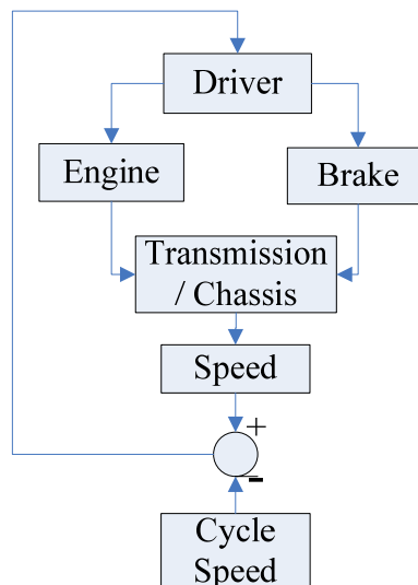
Figure 6-2 Forward Vehicle Modeling Algorithm in Dymola
