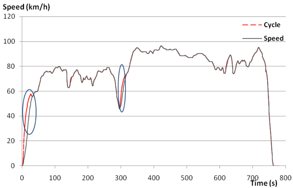
Figure 5-32 Vehicle Speed on HWFET Cycle
