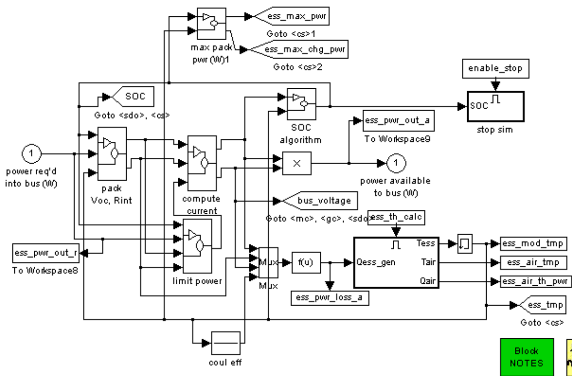
Figure 4-12 Energy Storage System Model in ADVISOR
