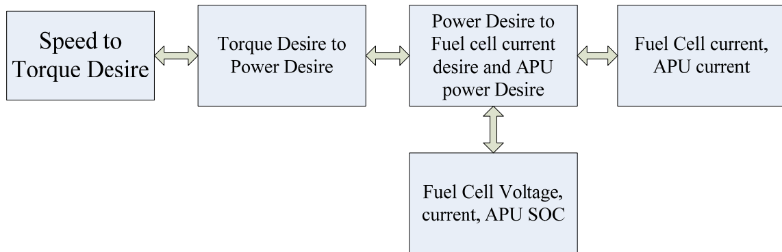
Figure 4-1 Elevator Powertrain Model
