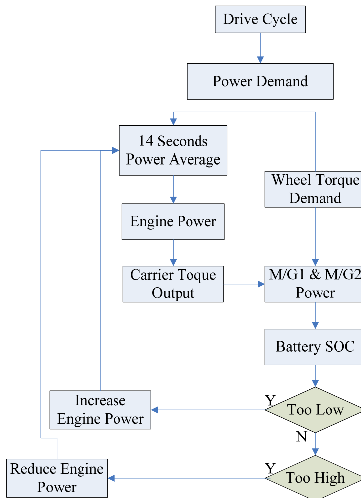
Figure 5-28 Power Management Chart Mode 2
