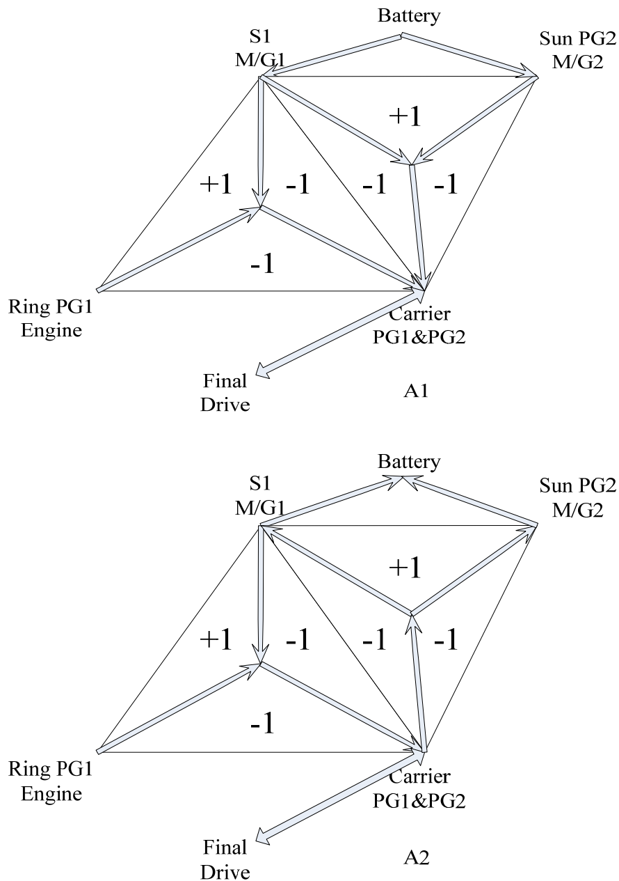
Figure 5-15 Power Flow of Second Mode at Vehicle Speed of V_{s3} or Lower
