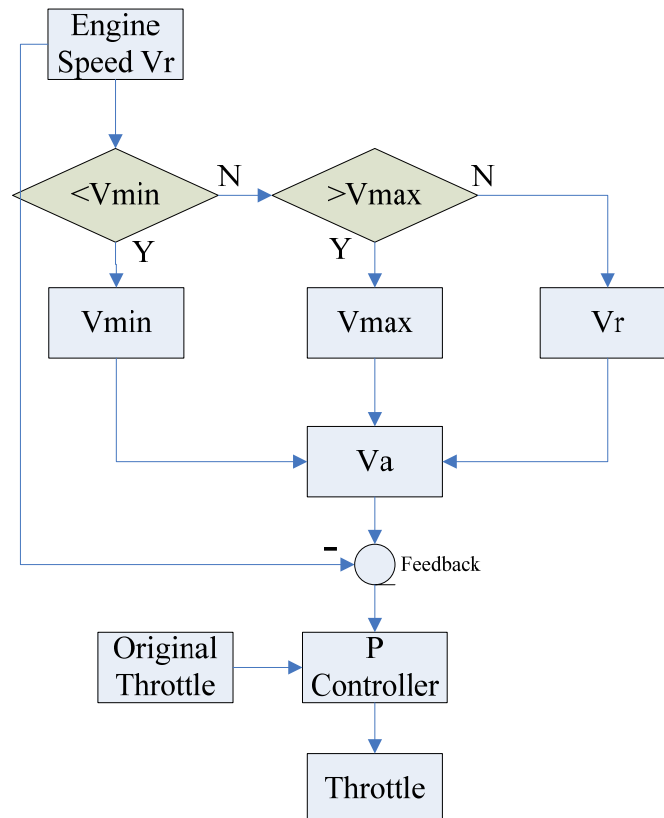
Figure 6-5 Engine Speed Governor Modeling
