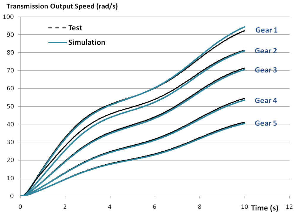
Figure 6-13 Transmission Model Validation - Output Speed
