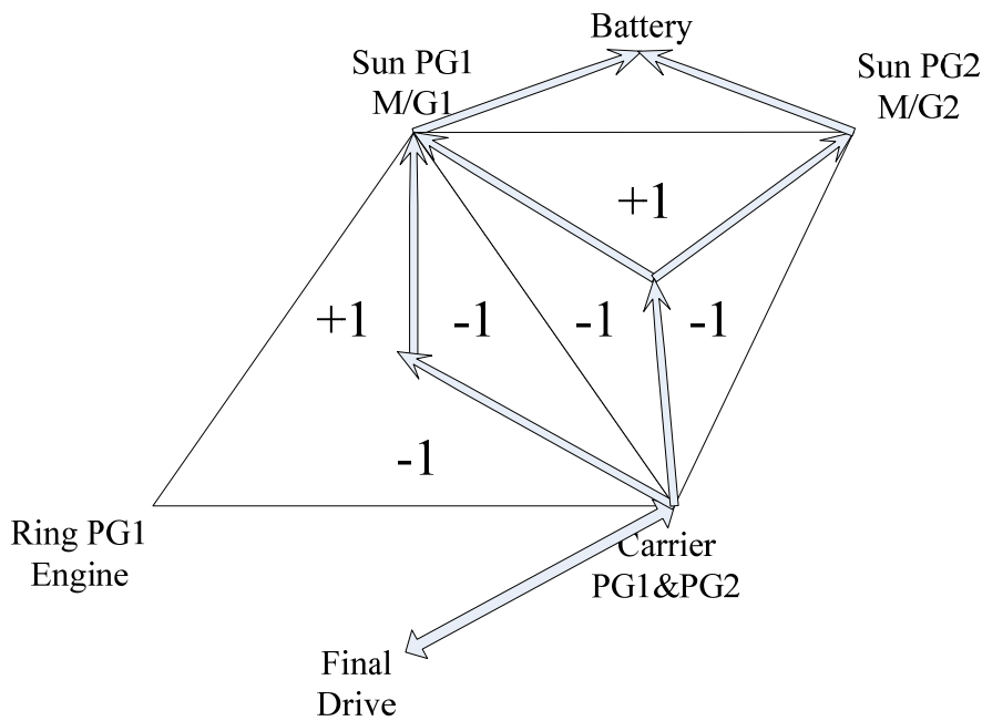
Figure 5-16 Power Flow of Second Mode during Brake at a Vehicle Speed of Vs3 or Lower
