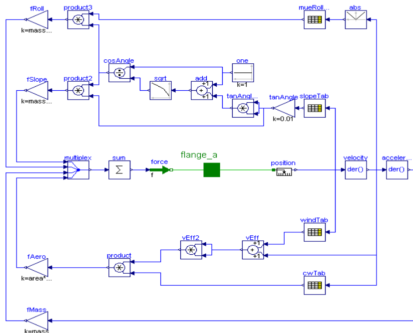
Figure 6-8 Vehicle Resistance Model
