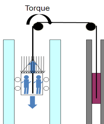
Figure 4-3 Physical Model of an Elevator
