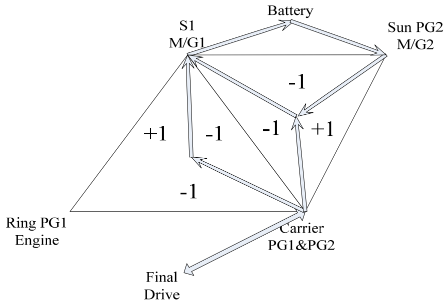
Figure 5-18 Power Flow of Second Mode Brake at Speed over V_{s3}
