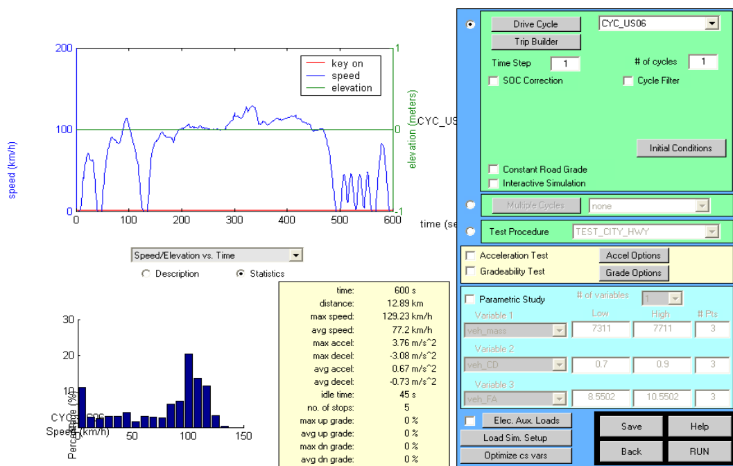
Figure 3-4 Simulation Setup Interface
