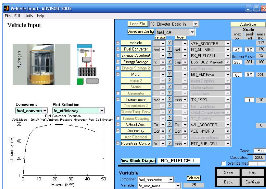
Figure 3-3 ADVISOR Vehicle Input Interface
