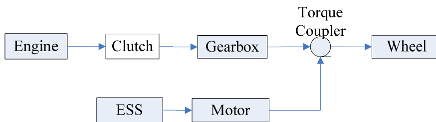
Figure 1-6 a Post-Transmission Parallel HEV Configuration
