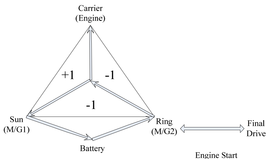
Figure 5-6 THS Power Flow Chart Engine Start
