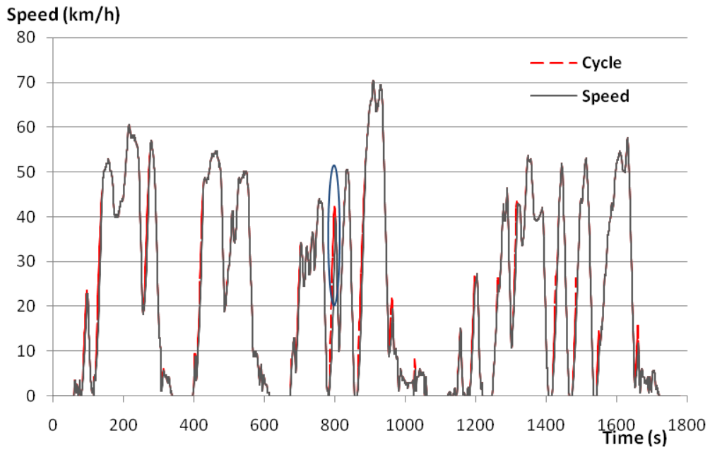
Figure 5-31 Vehicle Speed on CSHVR Cycle
