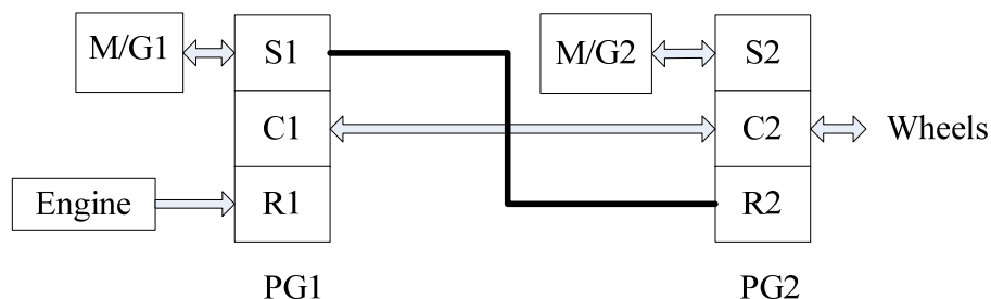
Figure 5-14 Second Mode Drivetrain Configuration
