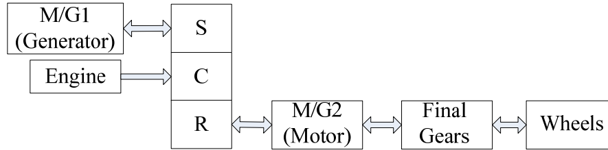
Figure 5-3 Toyota THS Configuration
