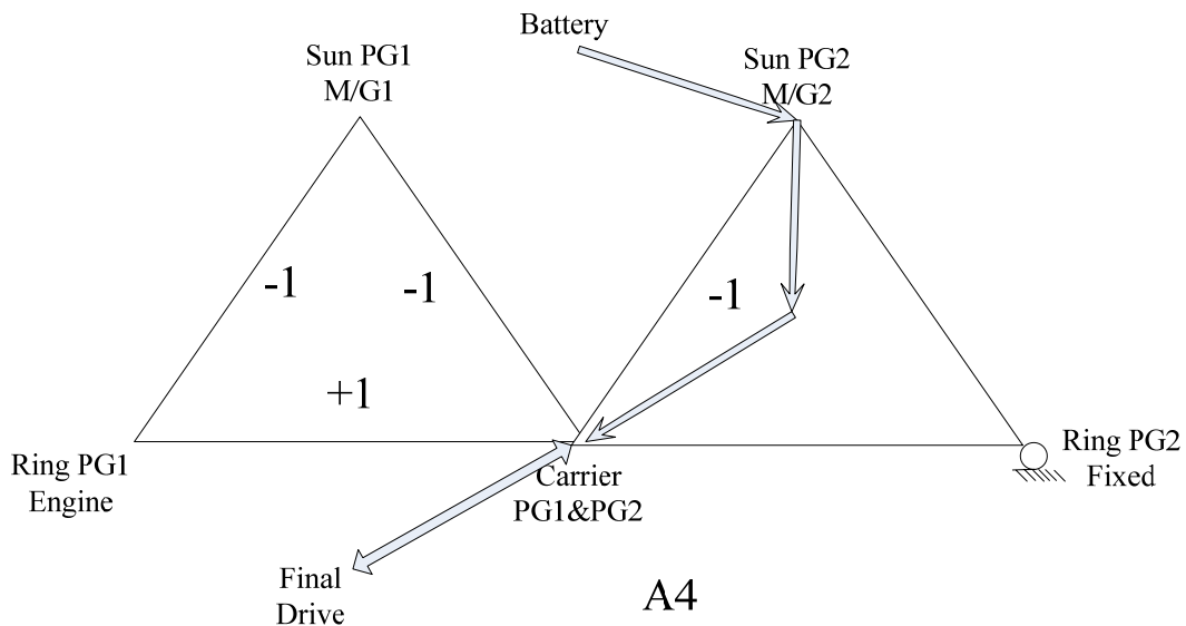
Figure 5-13 Power Flow Chart of Backward Movement in the First Mode
