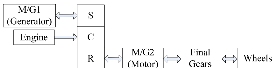
Figure 1-8 Toyota THS Configuration
