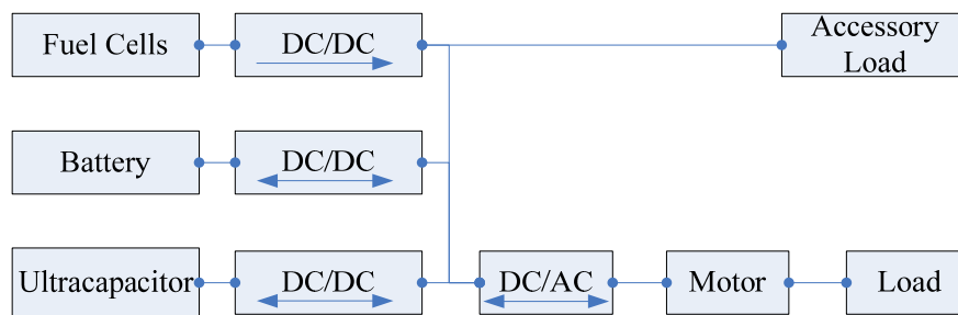
Figure 4-13 Power Management System of a Fuel Cells Hybrid Powertrain
