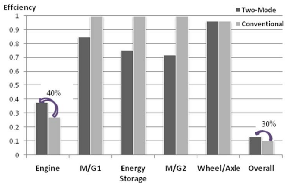
Figure 5-39 Efficiency of Two Mode HEV and Conventional ICE Vehicle on CSHVR Cycle
