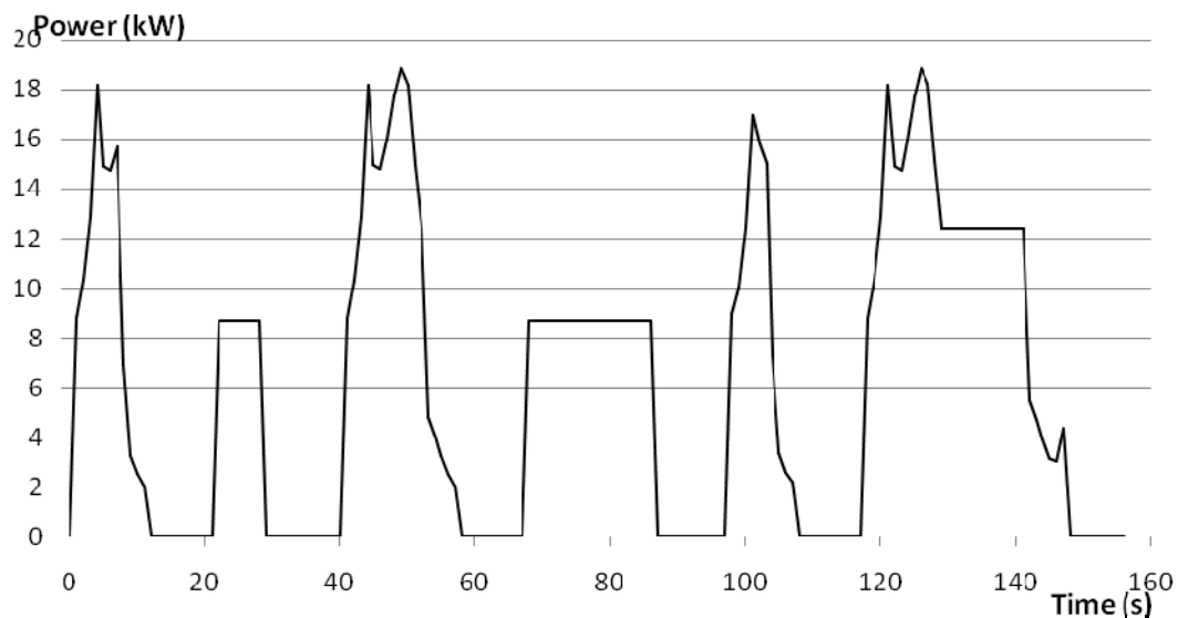
Figure 4-16 System Power Demand-Low Power Cycle
