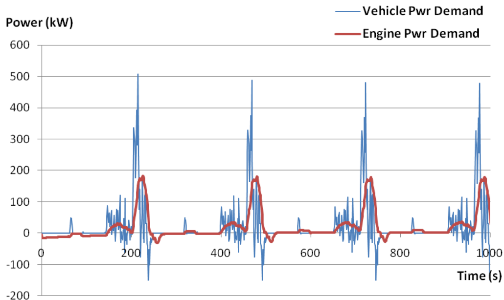
Figure 5-33 Engine Power on NYCCTRUCK Cycle
