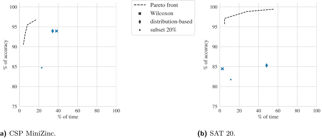
■ Figure 5 Percentage of accuracy with over median running time for the ranking-based selector. The Pareto front represents the front obtained from our results in Section 6.1. y-axis : percentage over all ordered pairs of algorithms in the dataset. x-axis : time spent running the new algorithm.
