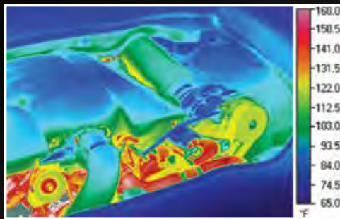
Underhood thermal image shown above. See pages 30-31 for additional information and thermal images.
