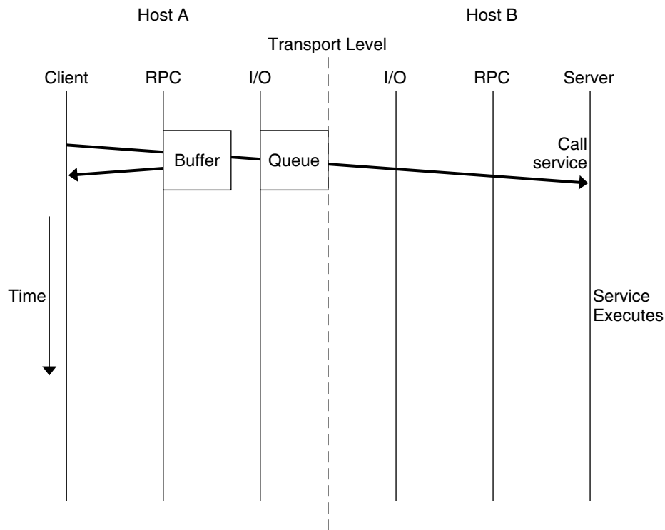
FIGURE 8-3 Non-Blocking Messaging
