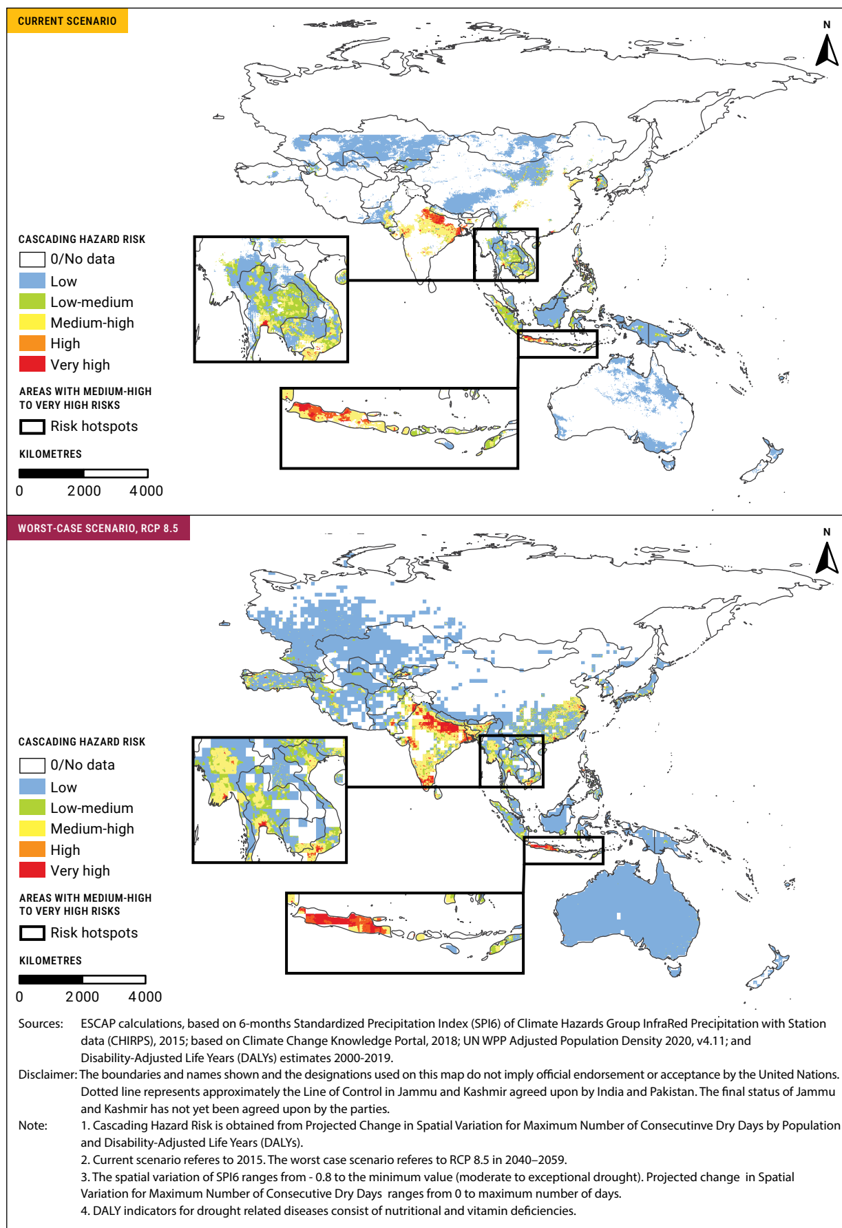
FIGURE 3-8 Population exposure to drought and related diseases under current and worst-case (RCP 8.5) scenarios in South-East Asia
