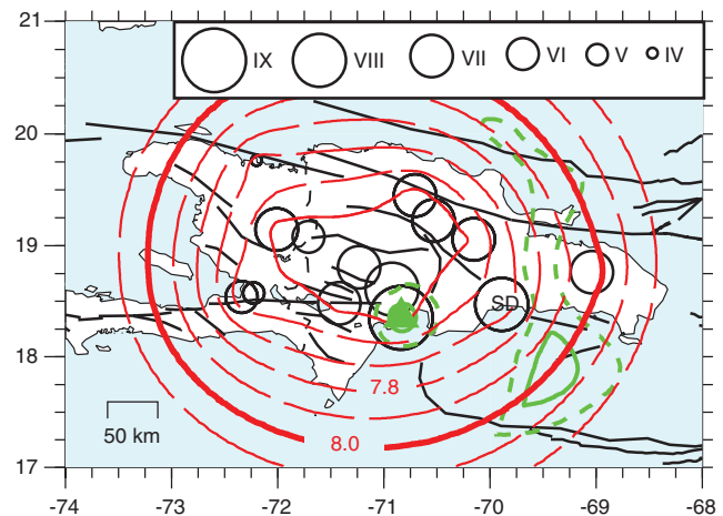
Figure 5. The 18 October 1751 earthquake with the preferred intensity assignments. The black circles are sites with MMI assignments with symbol size increasing with intensity. The black lines are active fault traces. The intensity center is a green filled triangle. Contours of M_1 are dashed red lines. The rms ( M_1 ) contour corresponding to the 67% and 95% confidence contours for location (Bakun and Wentworth, 1999) are shown as solid and dashed green lines, respectively. The SD marks the location Santo Domingo.
