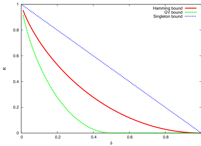
Figure 4.4: The Hamming, GV and Singleton bound for binary codes.
