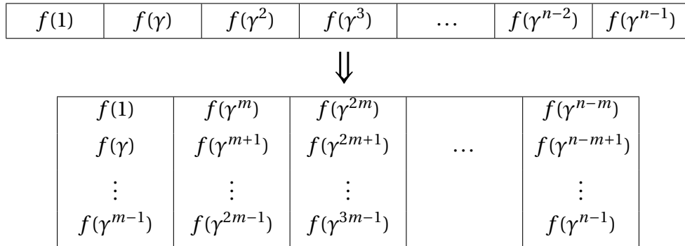
Figure 17.3: Folded Reed-Solomon code for general m \geq 1 .
