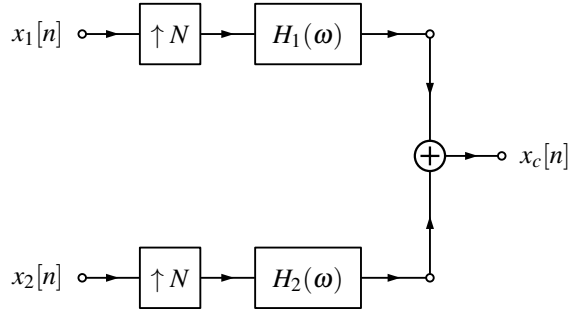
Figure 8: Filterbank reconstruction scheme
