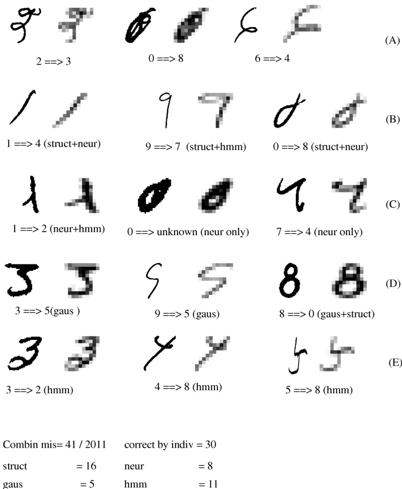
Fig. 4. Samples misclassified by the sum-rule combiner. (a) Samples not classified correctly by any individual classifier. (b) Samples classified correctly by the structural classifier. (c) By the Neural Network classifier. (d) By the Gaussian classifier. (e) By the HMM classifier.
