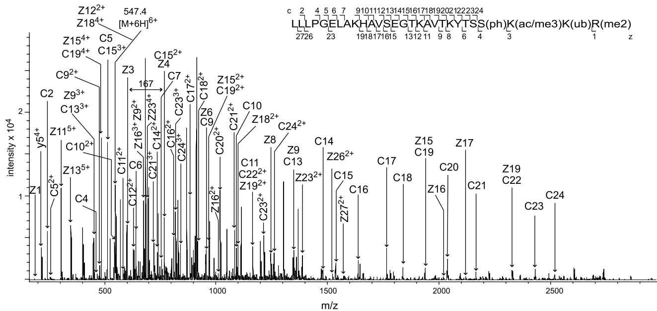
Figure 3. C-terminal peptide sequence of HIST1H2BN. ETD spectrum of the ion (M+6H)^{6+} at m/z 547.4 corresponding to the peptide with amino acids 101–128 in HIST1H2BN (GI: 119623520). The positions of z,y (C-terminal) and c (N-terminal) fragment ions are indicated in the spectrum and in the corresponding peptide sequence, where the lower case (ph), (ac/me3), (ub) and (me2) designate modifications of the amino acids by phosphorylation, acetylation/trimethylation, ubiquitination and dimethylation, respectively. doi:10.1371/journal.pone.0015960.g003
