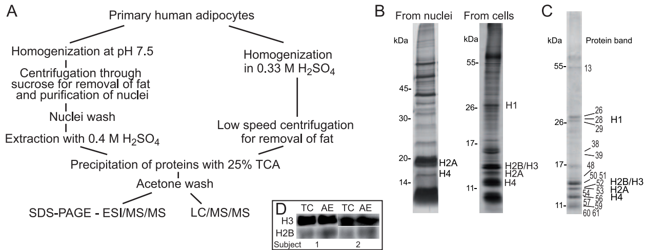
Figure 1. Comparison of histone preparations from nuclei and from whole cells. (A) A scheme for histone preparations from nuclei (left) and via whole cell extraction (right). (B) Silver stained SDS-PAGE gels with proteins extracted from nuclei and separated on a 14% acrylamide gel (left), and proteins extracted from whole cells and separated on a 12% acrylamide gel (right). Protein bands were cut out and in-gel digested with trypsin, the peptides were analyzed using ESI-MS/MS. Identified histones are indicated to the right. (C) Coomassie stained SDS-PAGE gel with proteins extracted from whole cells showing protein bands identified by MS/MS after in-gel digestion with trypsin. The numbers to the right indicate positions of the bands and histones as it specified in the Table 1. Molecular masses of reference proteins are indicated to the left of the gels in B and C. (D) Western blots showing efficiency of the direct acid extraction of histones from the cells by comparing immunoresponse of the samples corresponding to the equal amounts of total cell (TC) and acid extract (AE) from two different subjects. The antibodies against H3 and H2B were used, as indicated.
