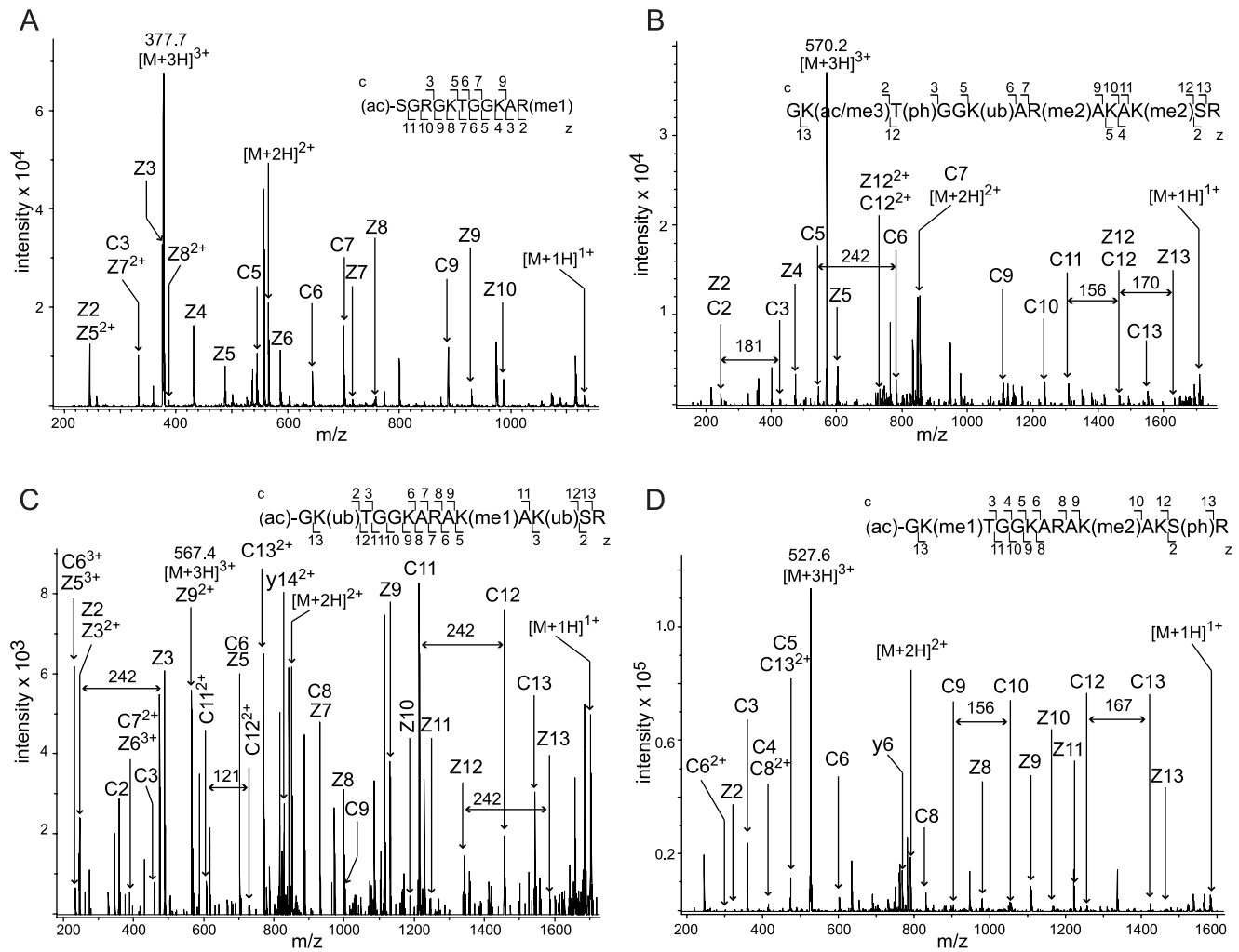
Figure 4. Identification of alternative processing of histone variant H2AFX. ETD fragmentation spectra corresponding to four differentially processed and modified N-termini of the isoform H2AFX (GI: 4504253). The positions of z,y (C-terminal) and c (N-terminal) fragment ions are indicated in the spectra and in the presented peptide sequences with the lower case (ac), (ac/me3) (me1), (me2), (ph) and (ub) corresponding to modifications of the amino acids by acetylation, acetylation/trimethylation, monomethylation, dimethylation, phosphorylation and ubiquitination, respectively. (A) ETD spectrum of the ion (M+3H)^{3+} at m/z 377.7 corresponding to the peptide with the amino acid positions 2–12 in H2AFX. The initial methionine has been removed, the N-terminal serine acetylated and the arginine in the peptide was monomethylated. (B) ETD spectrum of the peptide corresponding to the amino acid positions 5–18; the ion (M+3H)^{3+} at m/z 570.2. The peptide is modified by acetylation/trimethylation, phosphorylation, ubiquitination and two dimethylations. The mass difference of 181 between the fragment ions c3 and c4 corresponds to the phosphorylated threonine. The mass difference of 242 between the fragment ions c5 and c6 corresponds to the ubiquitinated lysine. The mass difference of 156 between the fragment ions c11 and c12 corresponds to the dimethylated lysine. The mass difference of 170 between the fragment ions z12 and z13 corresponds to the acetylated/trimethylated lysine. (C) ETD spectrum of the peptide corresponding to the amino acid positions 5–18; the ion (M+3H)^{3+} at m/z 567.4. The initial glycine has been acetylated after cleavage of the four N-terminal amino acids of the protein. The peptide is also modified by a monomethylation and two ubiquitinations. The mass differences of 242 between the fragment ions z2 and z3, z12 and z13 and c11 and c12, as well as the mass difference of 121 between the doubly charged fragment ions c11 2+ and c12 2+ correspond to the ubiquitinated lysines. (D) ETD spectrum of the peptide corresponding to the amino acid positions 5–18; the ion (M+3H)^{3+} at m/z 527.6. The N-terminal glycine is acetylated. The peptide is also modified by monomethylation, phosphorylation and dimethylation. The mass difference of 156 between the fragment ions c9 and c10 corresponds to the dimethylated lysine. The mass difference of 167 between the fragment ions c12 and c13 corresponds to the phosphorylated serine. doi:10.1371/journal.pone.0015960.g004
