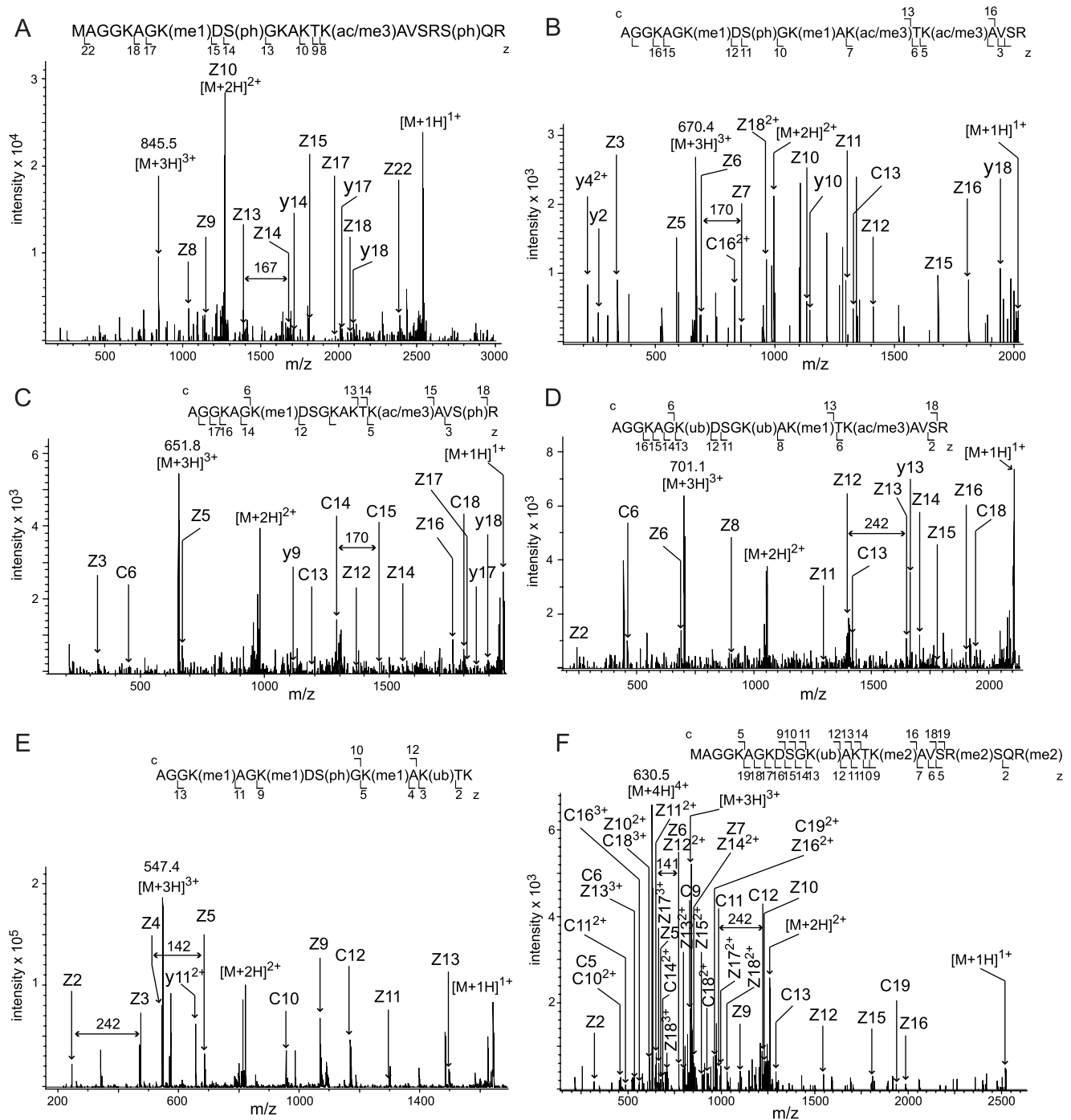
Figure 2. Differentially processed and modified N-termini of histone H2AFZ. ETD fragmentation spectra corresponding to six differentially processed N-terminal peptides of the variant H2AFZ (GI: 4504255). A–E show peptides identified in the histone analysis optimization process, while F presents the spectrum of the peptide identified during the following nanoLC/MS/MS analysis of six different subjects. The positions of zy (C-terminal) and c (N-terminal) fragment ions are indicated in the spectra and in the presented peptide sequences with the lower case (ac/me3) (me1), (me2), (ph) and (ub) corresponding to modifications of the amino acids by acetylation/trimethylation, monomethylation, dimethylation, phosphorylation and ubiquitination, respectively. (A) ETD spectrum of the ion [M+3H]^{3+} at m/z 845.5 corresponding to the peptide with the amino acid positions 1–23 in H2AFZ. The peptide is modified by methylation, acetylation/trimethylation, and two phosphorylations. The mass difference of 167 between the fragment ions z13 and z14 corresponds to the phosphorylated serine at the position 10. (B) ETD spectrum of the peptide corresponding to the amino acid positions 2–20; the ion [M+3H]^{3+} at m/z 670.4. The peptide is modified by two monomethylations, two acetylations/trimethylations and a phosphorylation. The mass difference of 170 between the fragment ions z6 and z7 corresponds to the acetylated/trimethylated lysine at the position 13. (C) ETD spectrum of the peptide corresponding to the amino acid positions 2–20; the ion [M+3H]^{3+} at m/z 651.8. The peptide is modified by monomethylation, acetylation/trimethylation and phosphorylation. The mass difference of 170 between the fragment ions c14 and c15 corresponds to the acetylated/trimethylated lysine at the position 15. (D) ETD spectrum of the peptide corresponding to the amino acid positions 2–20; the ion [M+3H]^{3+} at m/z 701.1. The peptide is modified by two ubiquitinations, monomethylation and acetylation/trimethylation. The mass difference of 242 between the fragment ions z12 and z13 corresponds to the ubiquitinated lysine at the position 7. (E) ETD spectrum of the peptide corresponding to
