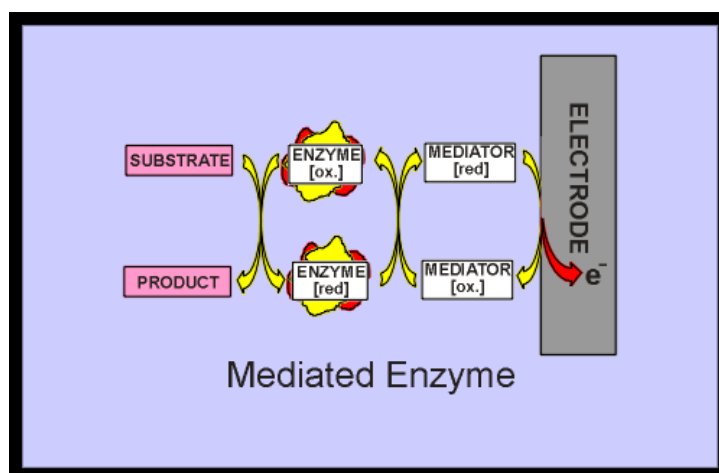
Figure 4: Mediated Biosensor Schematic
