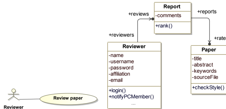
Fig. 2. The use case “review a paper” and its class model in UML-like notation.
