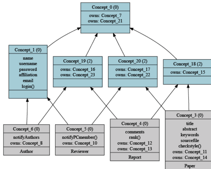
Fig. 6. The final “class lattice” where the concept \perp is omitted.
