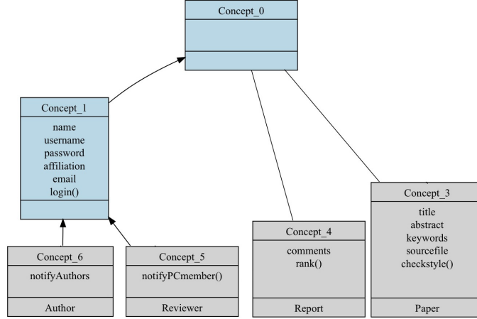
Fig. 4. The concept lattice \mathcal{L}_{\text{class}} corresponding to the formal context \mathcal{K}_{\text{class}} (Table 1) where the bottom concept \perp is omitted.
