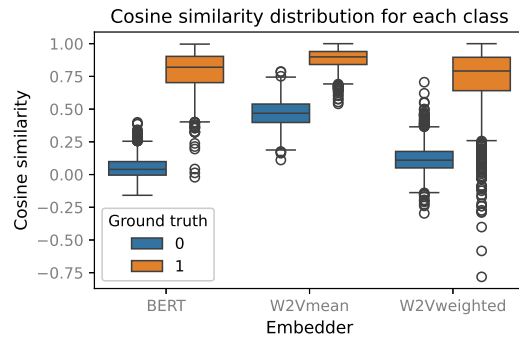
Figure 2: The distribution of results from BERT, mean aggregated Word2Vec and our solution grouped by ground truth similarity.
