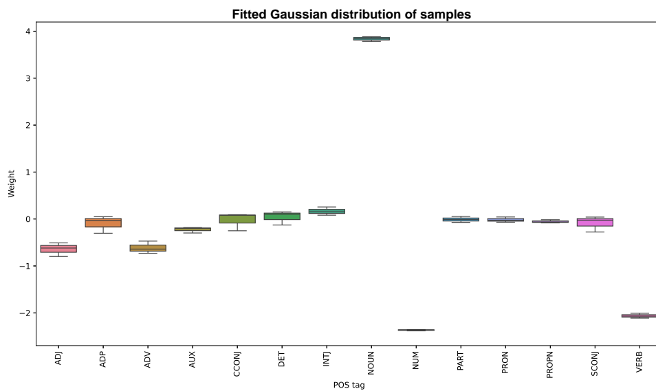
Figure 1: Fitted Gaussian distribution of samples
