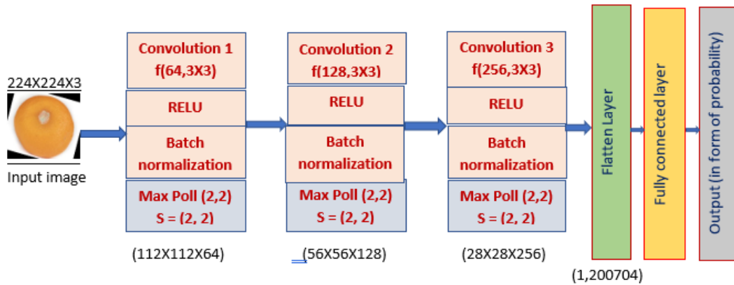
Figure 3: CNN architecture
