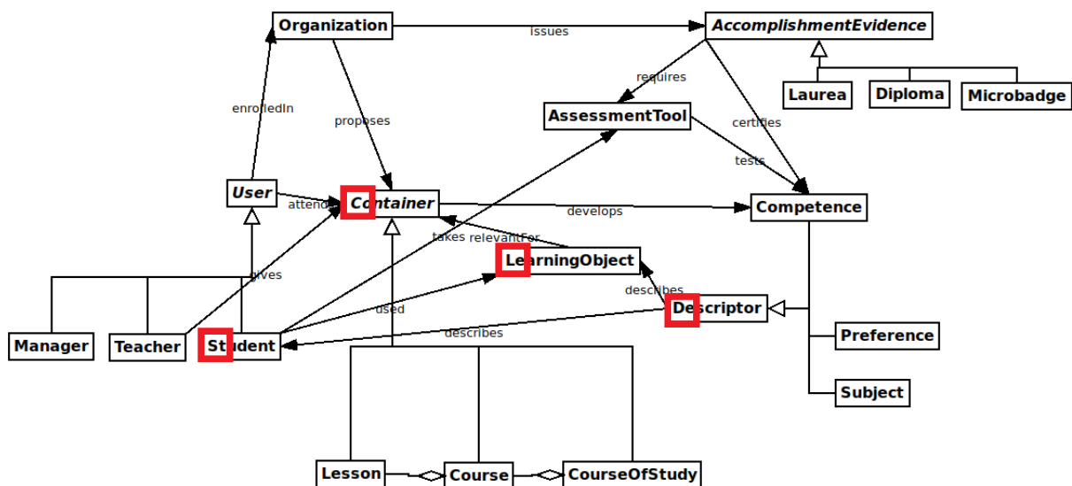
Figure 2: Portion of KEPLAIR's ontology. In red the classes used in the case study (see Section 4.2)
