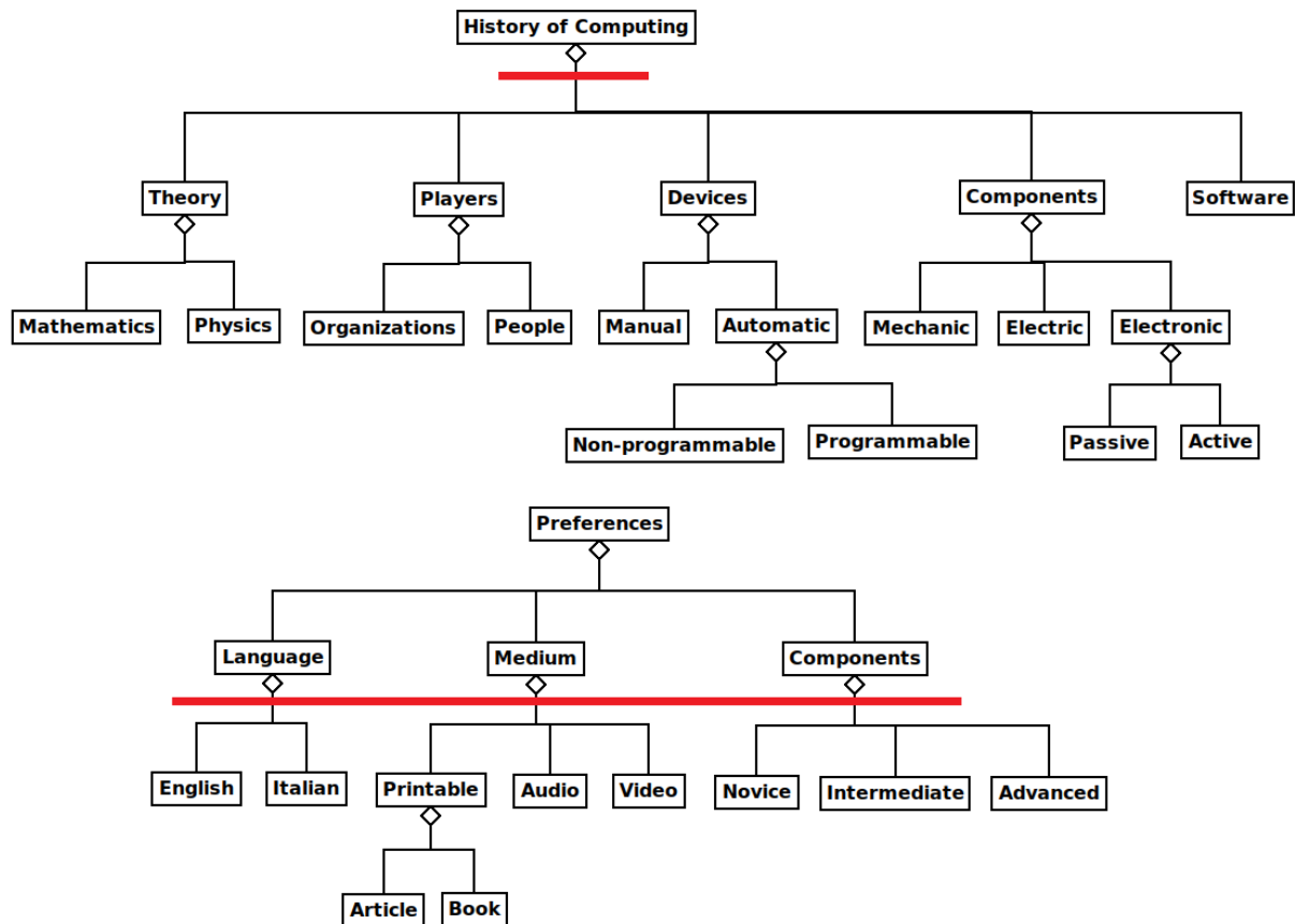
Figure 4: Fragment of descriptors taxonomy used in our experiment
