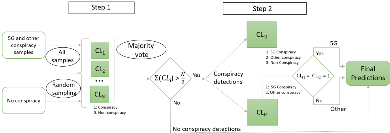
Figure 1: Our proposed pipeline for tackling the challenge of Corona virus and 5G conspiracy
