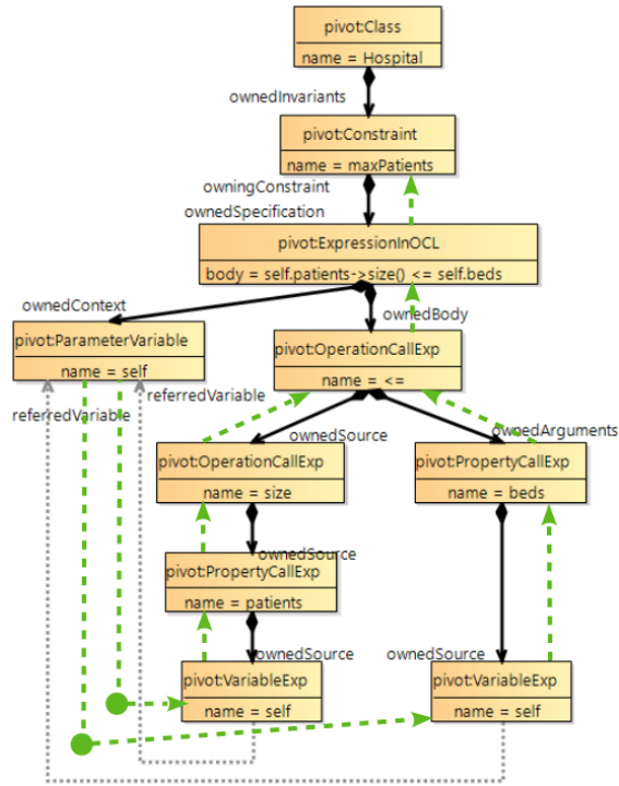
Fig. 6. Fixed Naive Visualization of vOCL invariant
