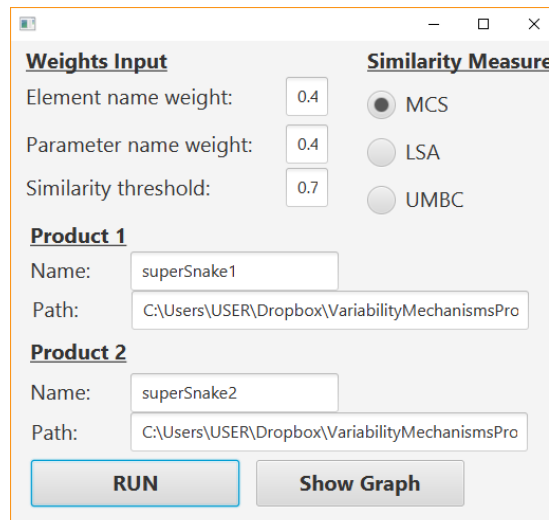
Figure 2. A screenshot of VarMeR inputs
