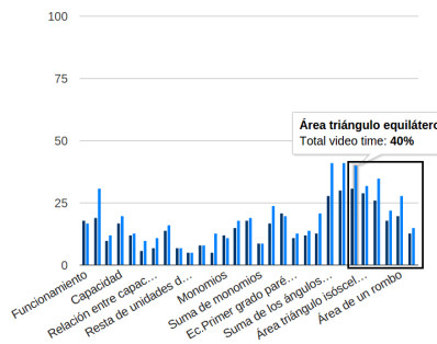
Figure 5. Video Time Watched visualization of the aggregate of all the students in the class.
