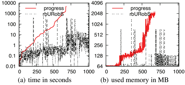
Figure 1: Comparison of regression-based uniform robustness search vs. a belief-state based progression approach. For readability, we sorted the test cases by the time of the latter.
