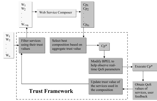
Figure 1: Our framework for considering trust while composing Web services.
