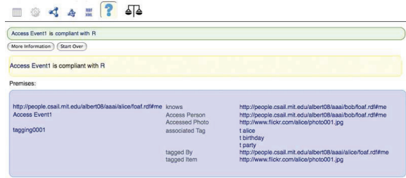
Figure 1: The Justification UI in Tabulator.
