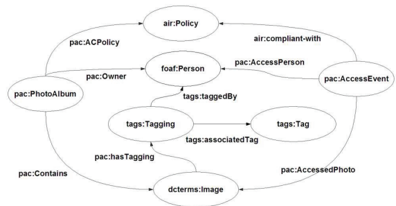
Figure 3: The Photo Access Control Ontology.
