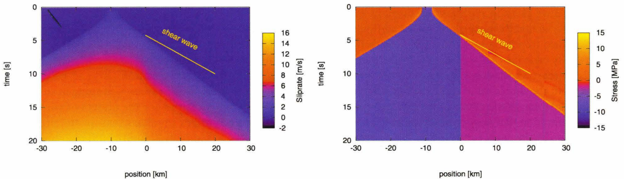
Plate 3. Numerical simulation of rupture propagation along the fault shown in Figure 6. The Figure on the top shows slip as a function of position along the fault and time. The bottom picture shows the corresponding stress field. The short yellow line shows the slope of a wave propagating at the shear wave speed. Rupture speed reduces significantly once the fault propagates beyond the beginning of zone of complex geometry.
