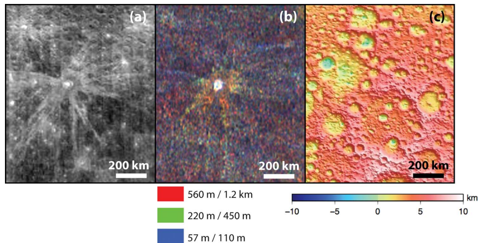
Figure 6. Lunar far-side crater Jackson and its ray system, centered at 19^\circ\text{E} and 22.4^\circ\text{N} , shown in (a) the 750 nm Clementine albedo map [e.g., McEwen and Robinson, 1997 ], (b) the median differential slope map, as in Figure 5, and (c) the topography [ Smith et al., 2010b ]. Rays of young, Copernican-age craters are clearly expressed as streaks of high albedo relative to the background. Though they do not add obvious relief to the topography, the rays are distinctly rougher at the \sim 220 m and \sim 560 m baselines compared to the highlands, making them appear yellow to orange in the composite roughness map.
