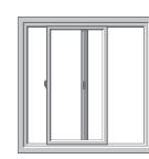
Sliding Window
