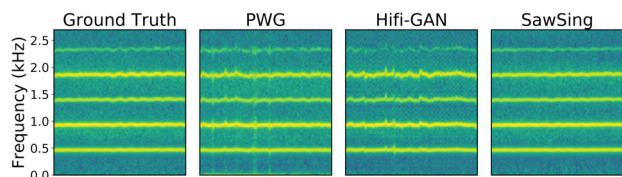
Figure 1: The magnitude spectrograms of a long utterance of an original recording (‘ground truth’) and those reconstructed by two widely-used neural vocoders, Parallel WaveGAN (PWG) [14] and HiFi-GAN [15], and the proposed SawSing. Each vocoder is trained on 3 hours of recordings from a female singer until convergence. We see glitches in the results of PWG and HiFi-GAN.
