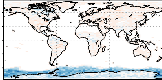
(f) Elevated smoke
