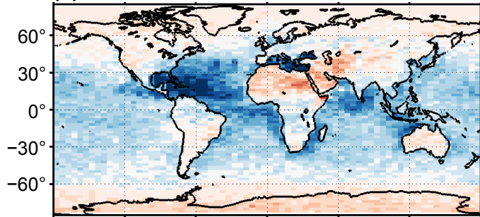
(e) Polluted dust
