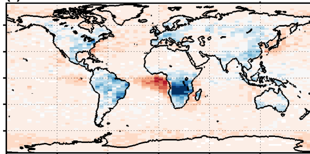
(f) Elevated smoke
