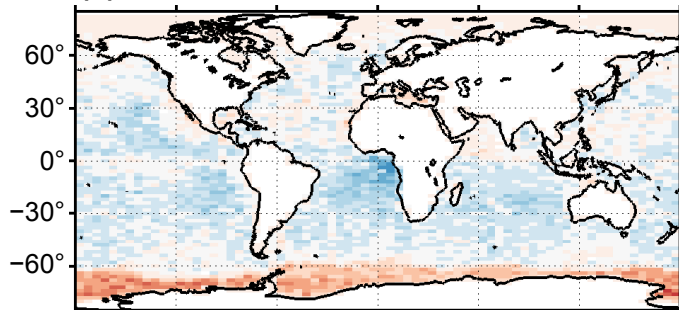
(c) Polluted continental / smoke
