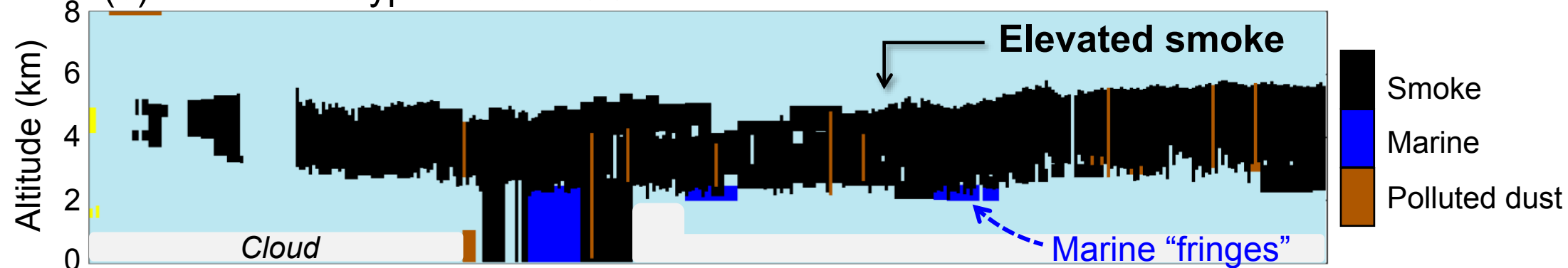
(c) Aerosol subtypes after SCAARF
