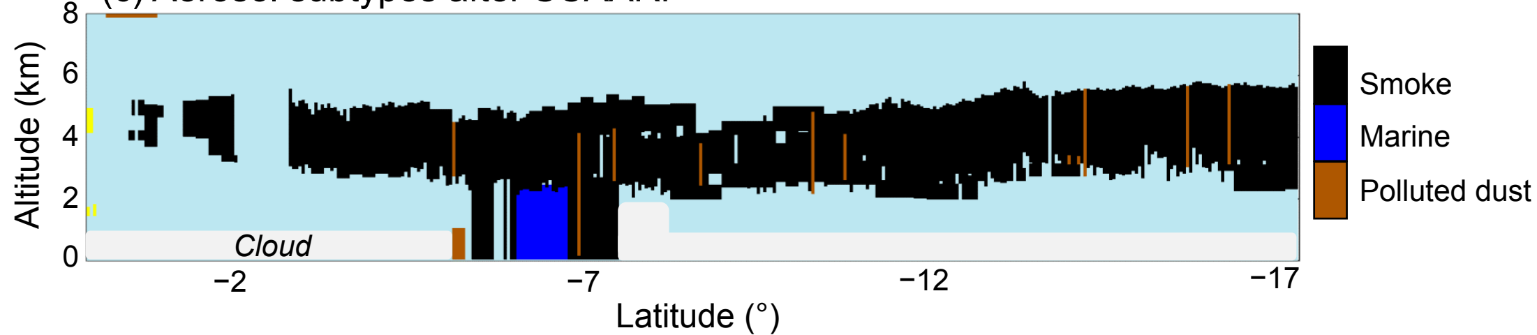
(c) Aerosol subtypes after SCAARF
